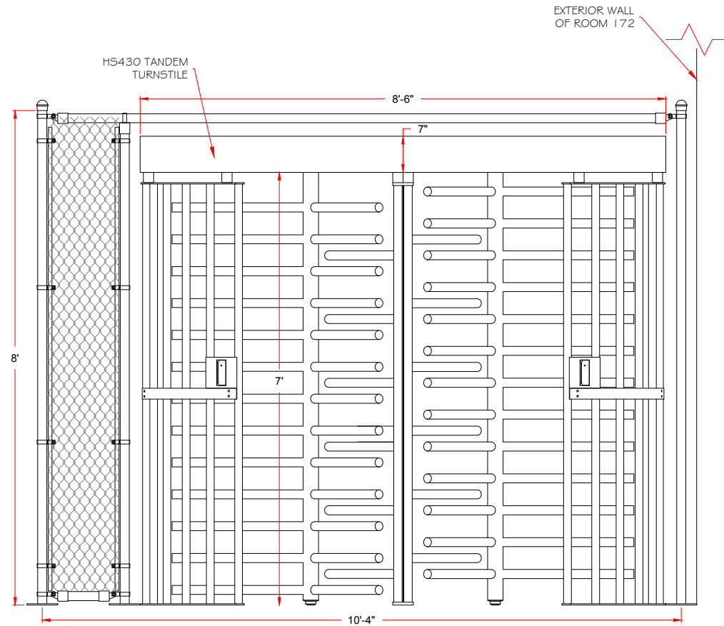
ELEVATION - Turnstile Side
