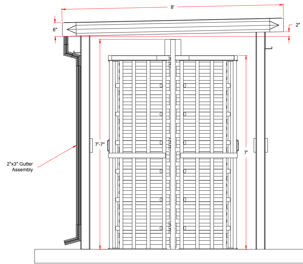
SIDE ELEVATION (heaters not shown)
