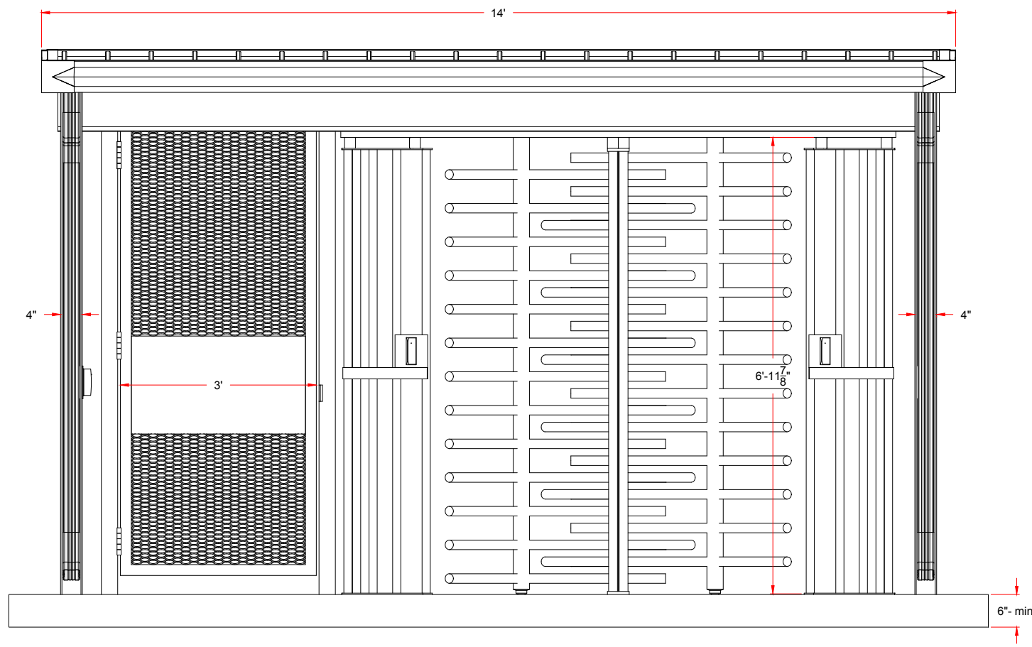
ELEVATION ENTRY SIDE
