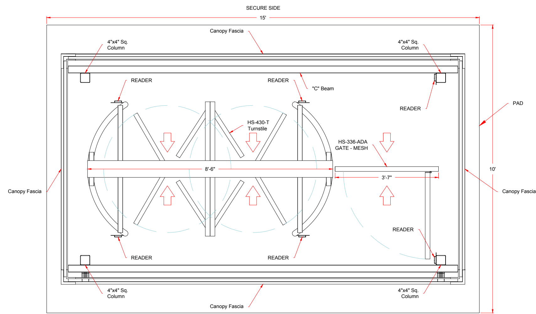
ENTRANCE SIDE FOOT PRINT (flat pan not shown)
