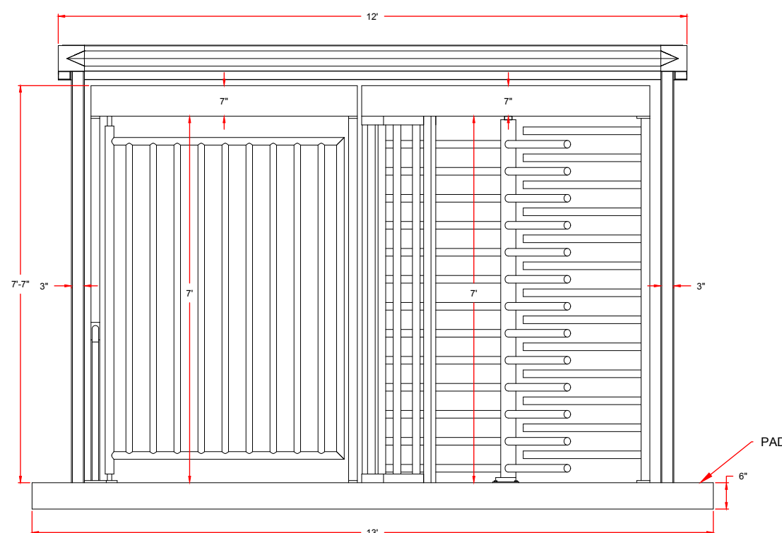
ELEVATION (secure side - C-Beam & Gutter not shown)
