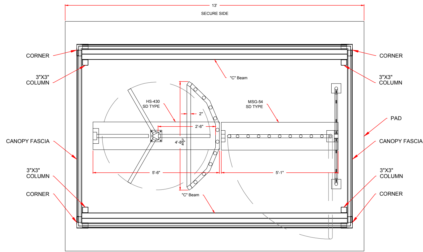
FLOOR PLAN (flat pan - gutter not shown)
