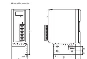
Two holes only for OP-51624.
