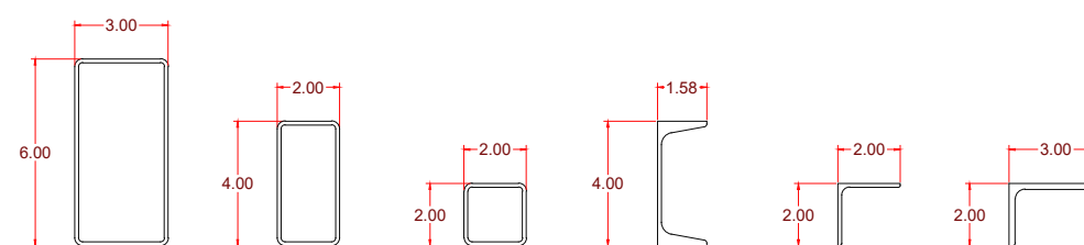
ANGLE, C - CHANNEL, & SQUARE TUBE PROFILES WITH DIMENSIONS
