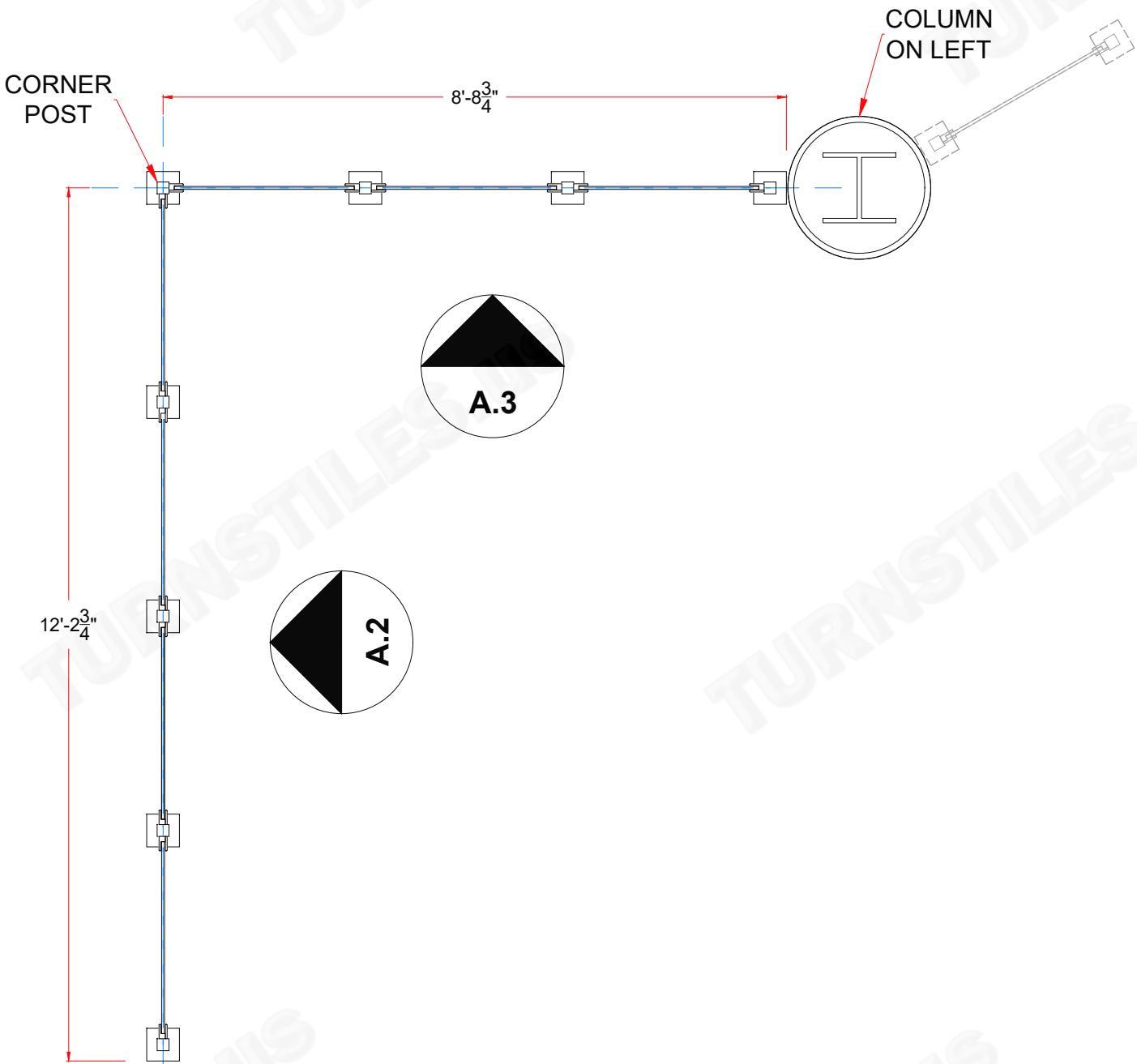
FLOOR PLAN
