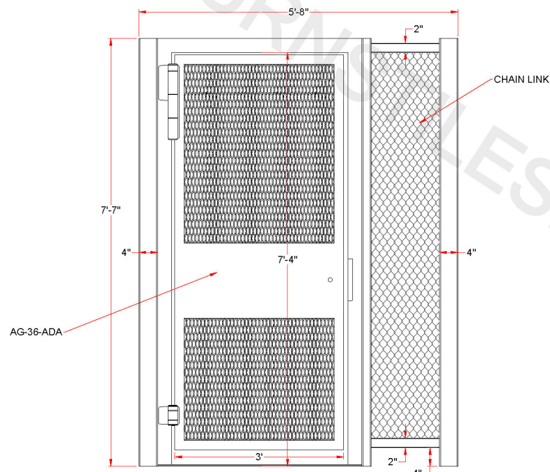
FRONT ELEVATION - UN-SECURE SIDE
