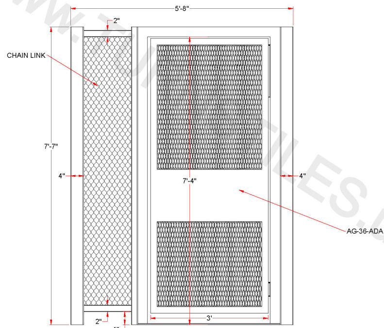
REAR ELEVATION - SECURE SIDE
