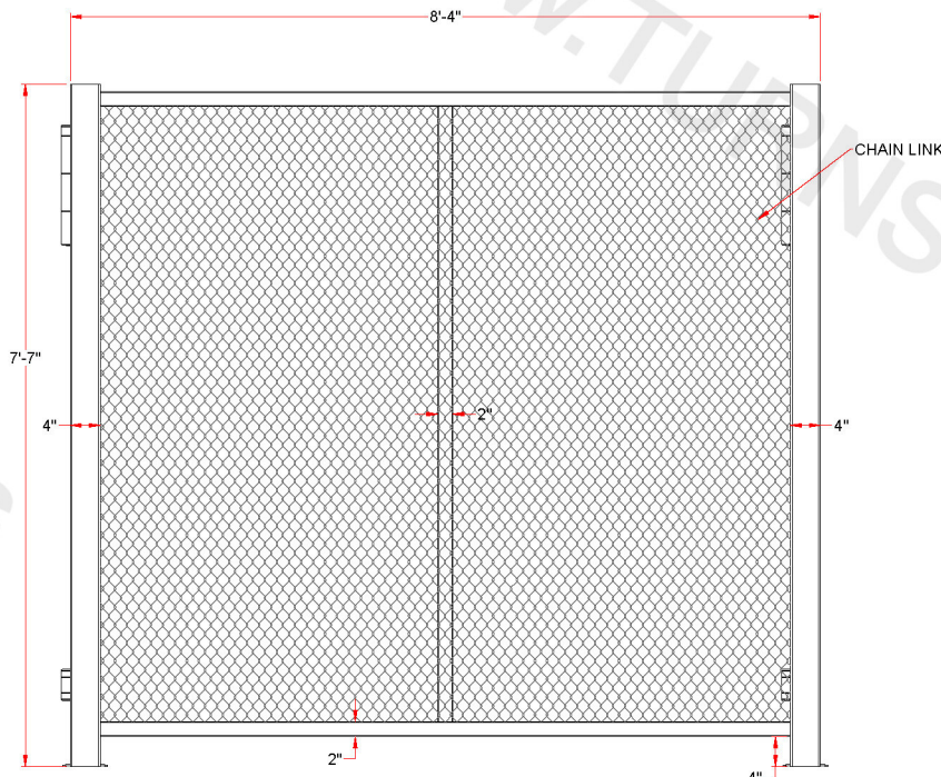
ELEVATION - RIGHT SIDE
