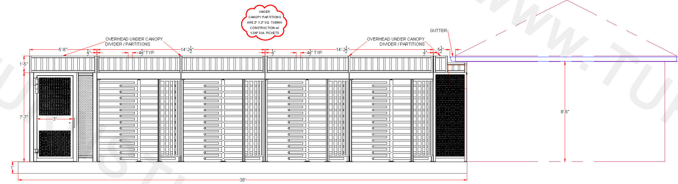
CONCRETE PAD - EQUIPMENT ELEVATION w/o CANOPY FACING NORTH
