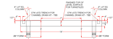
ELEVATION PAD SIDE CHANNEL DRAIN DETAIL - TBD
