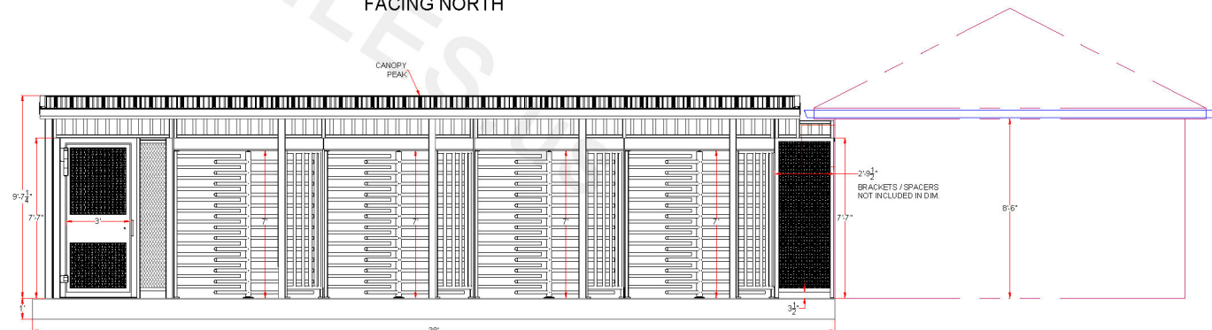
CONCRETE PAD - EQUIPMENT ELEVATION w/ CANOPY FACING NORTH
