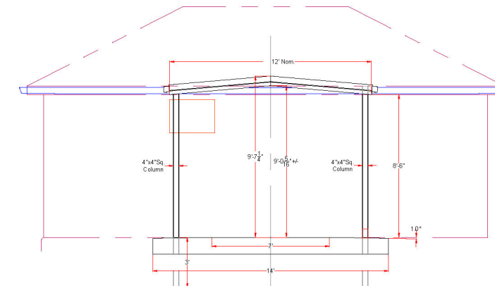
CONCRETE PAD - ELEVATION - CANOPY FACING WEST
