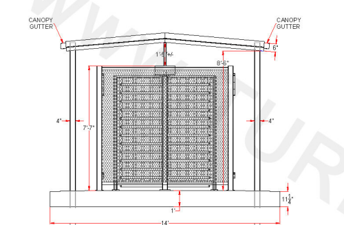
CONCRETE PAD - EQUIPMENT ELEVATION w/ CANOPY FACING WEST
