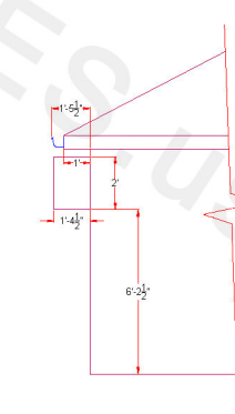
POST 2 BLDG - ELEVATION FACING NORTH - NO EQUIPMENT
