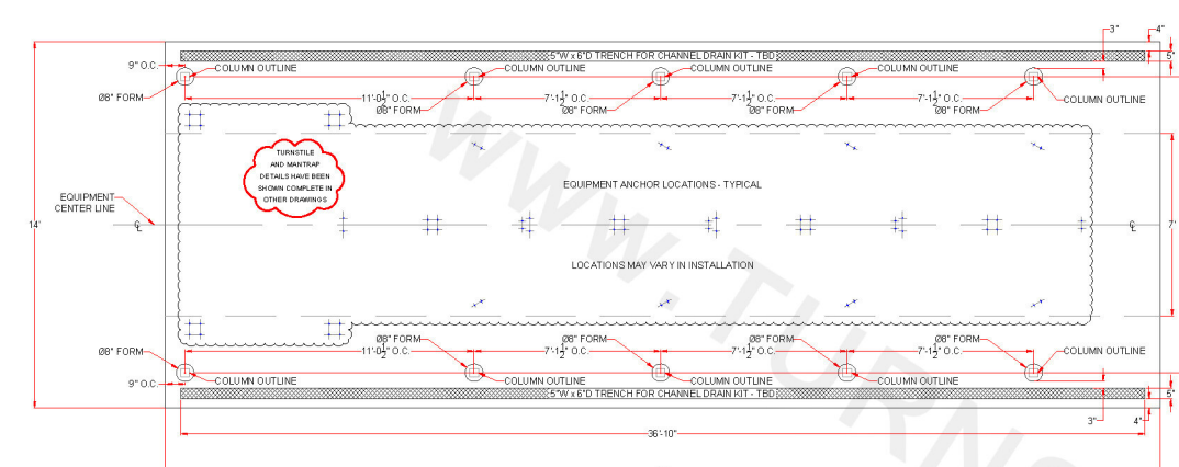
CONCRETE PAD - CANOPY COLUMN FORM AND EQUIPMENT ANCHOR LOCATIONS
