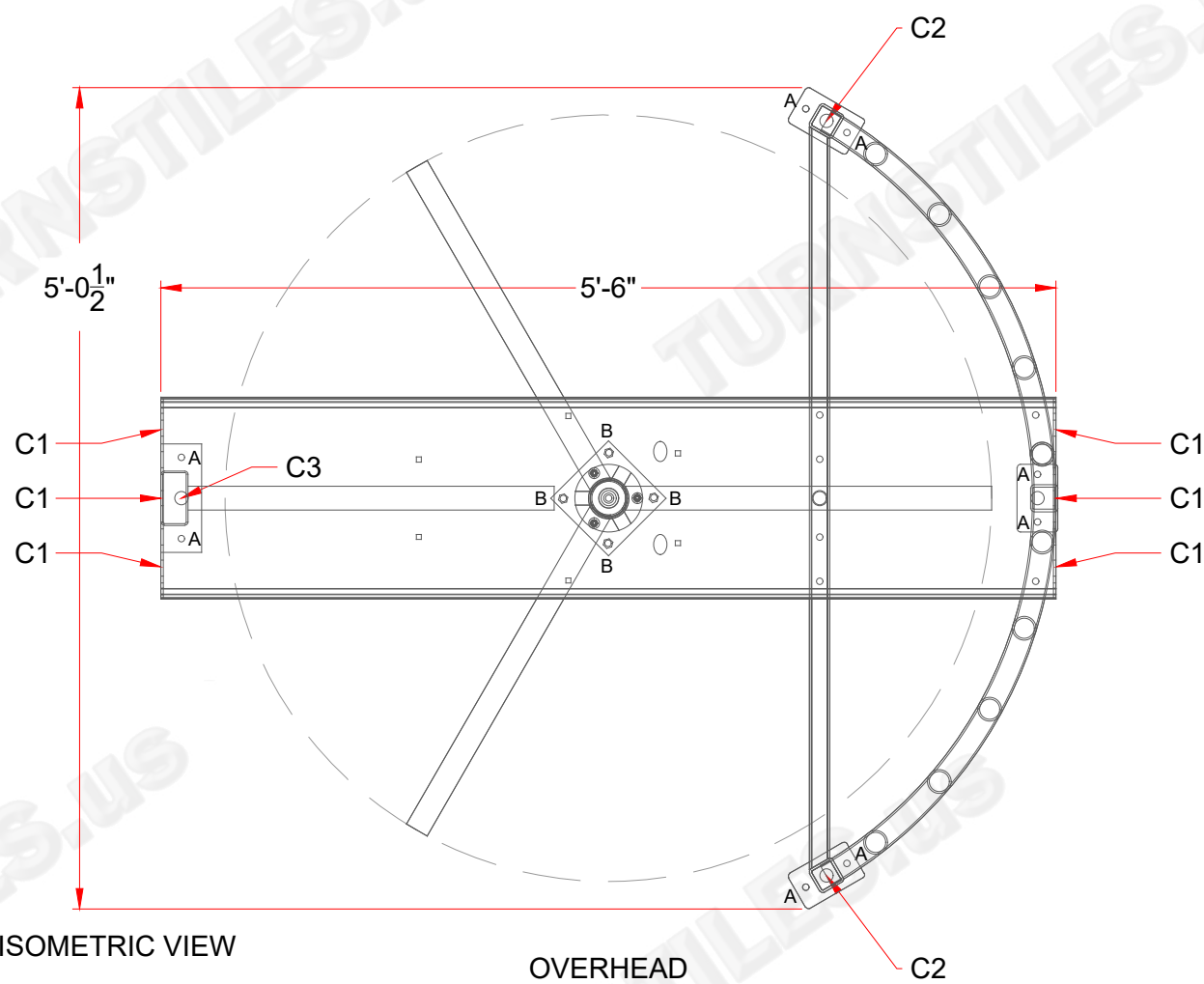
OVERHEAD
