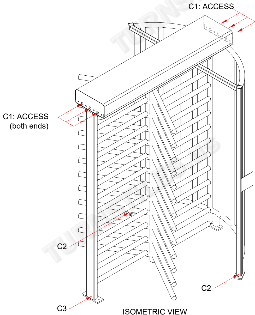
ISOMETRIC VIEW
