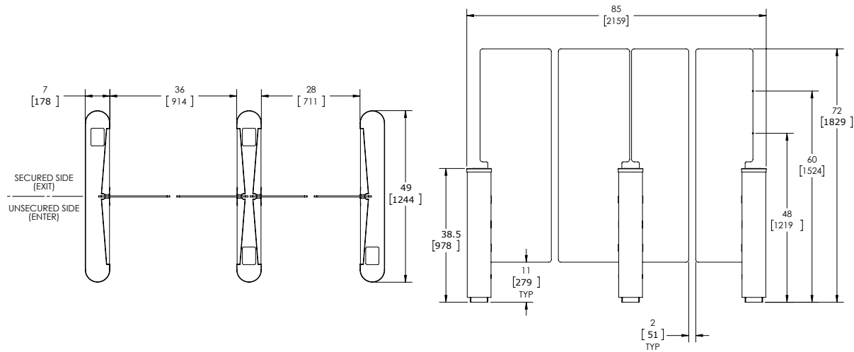
TYPICAL OBSG-HG-CV, ROUND ENDS ONE 28" STANDARD LANE ONE 36" ADA LANE
