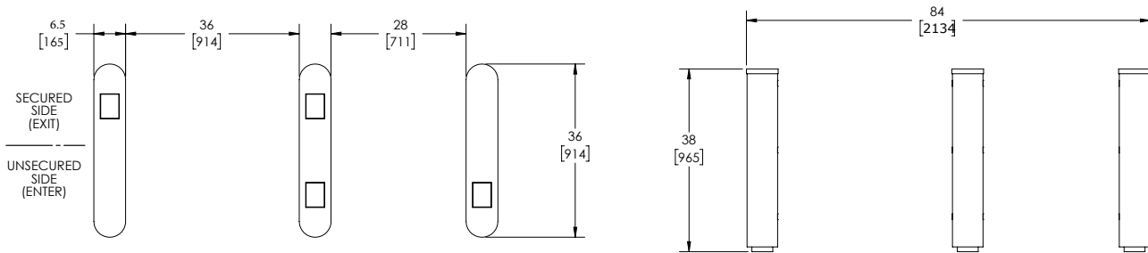
TYPICAL PONB-36-CV, ROUND ENDS ONE 28" STANDARD LANE ONE 36" ADA LANE 2 LANE 3 PED
