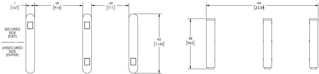
TYPICAL PONB-45, ROUND ENDS ONE 28" STANDARD LANE ONE 36" ADA LANE 2 LANE 3 PED
