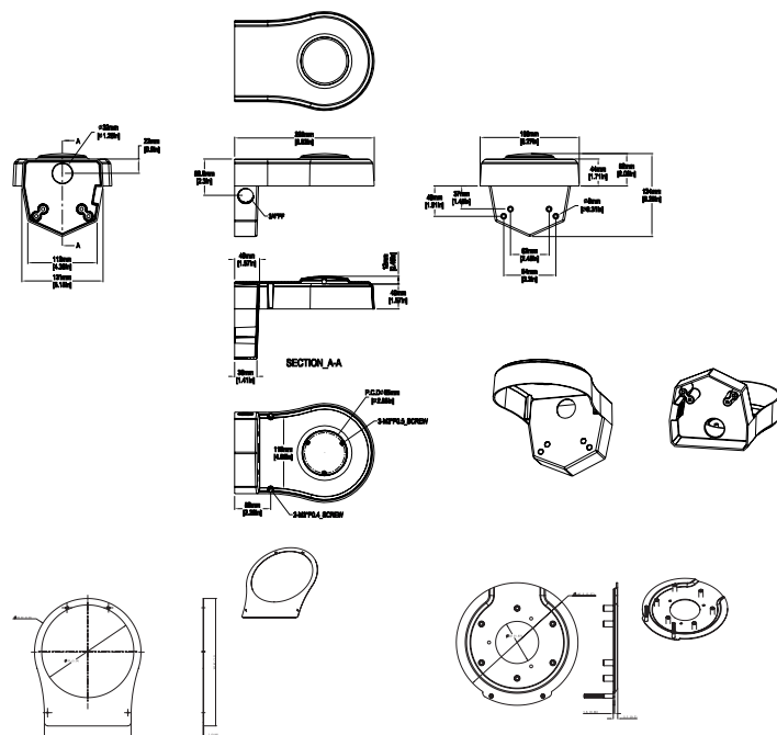
Illustra 600 wall mount adapter cover plate
