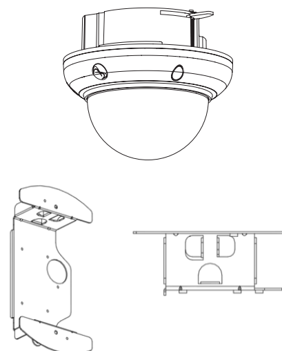
Recessed mount kit for outdoor mini-dome to maintain IP67 rating
