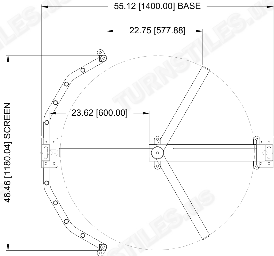
PLAN VIEW (SECTIONED)
