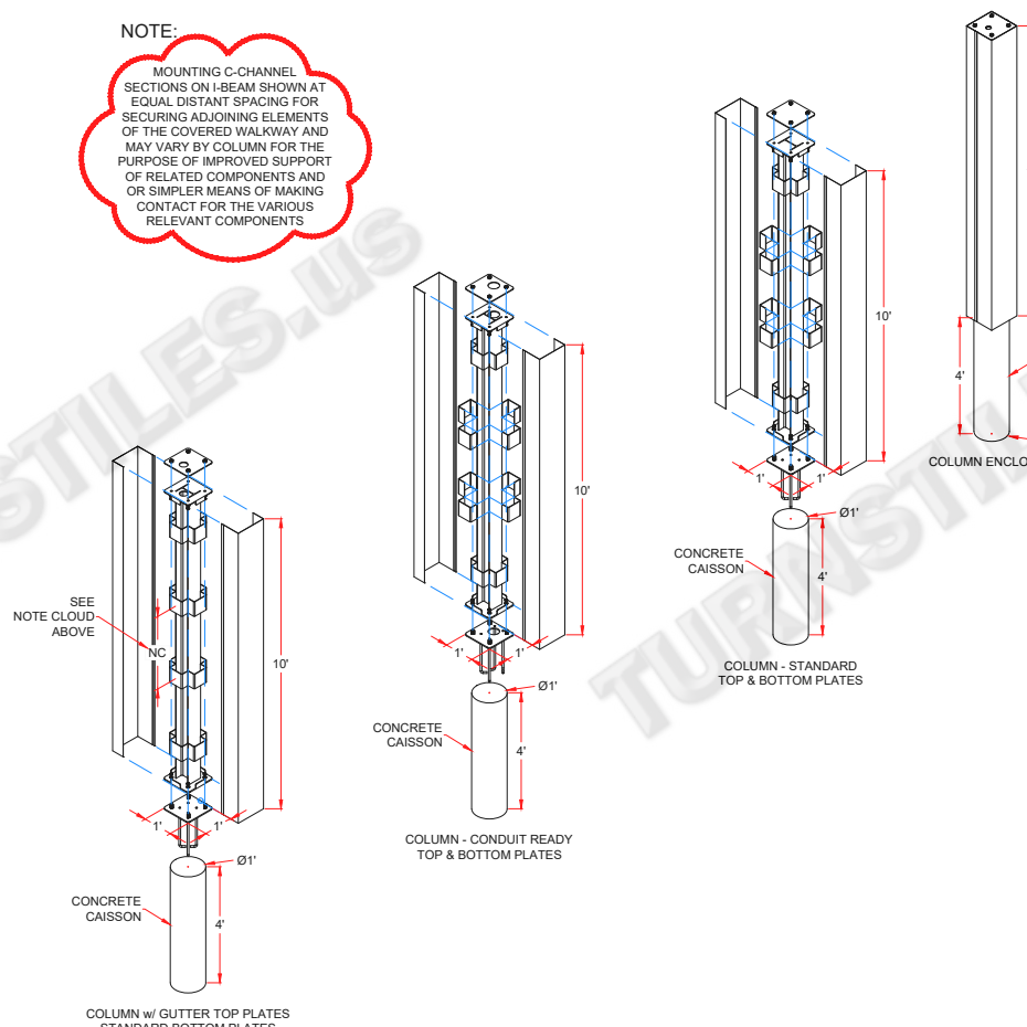
COLUMN INTERNAL DETAILS
