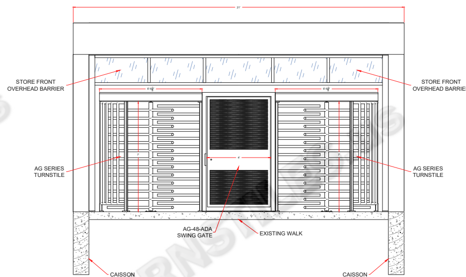
ELEVATION - TURNSTILES & SWING GATE
