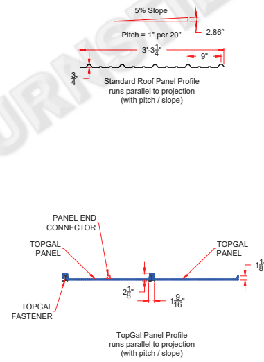
ROOFING TYPE(S) - PROFILES - DETAILS
