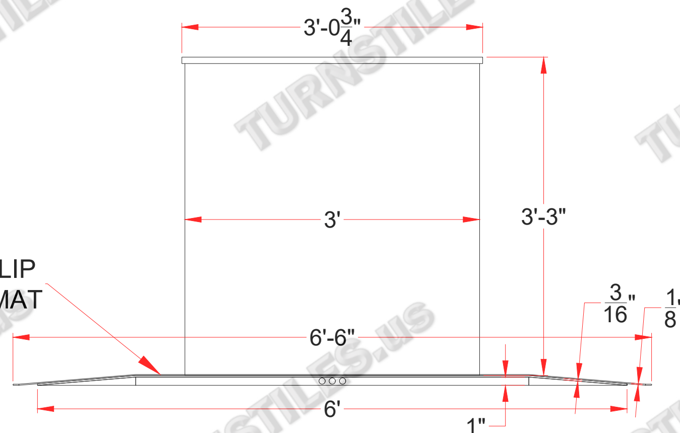
SIDE VIEW (reader & intercom not shown)
