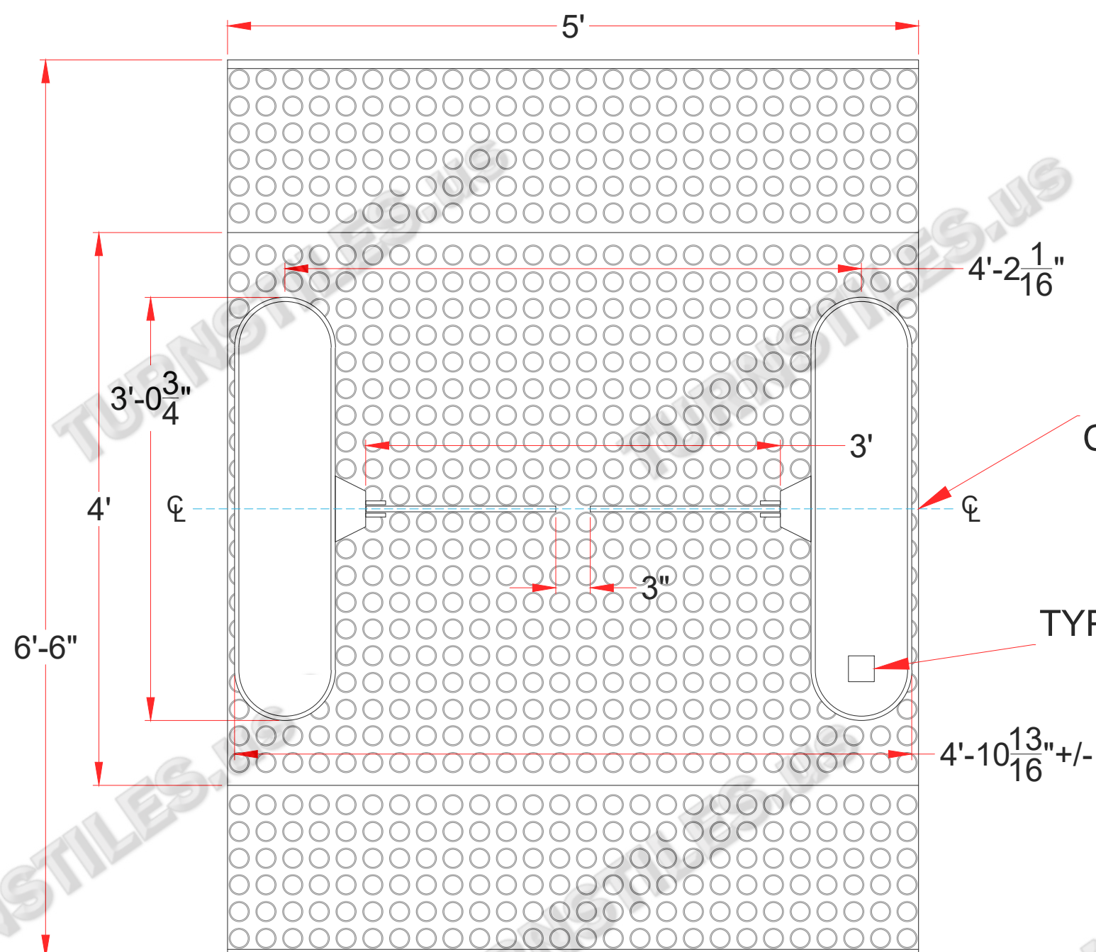
FLOOR PLAN (reader & intercom not shown)
