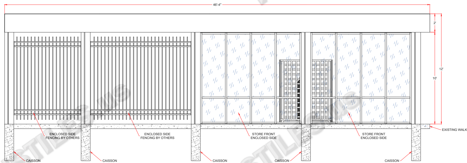
ELEVATION - LEFT SIDE
