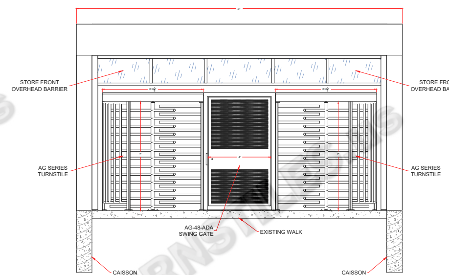
ELEVATION - TURNSTILES & SWING GATE
