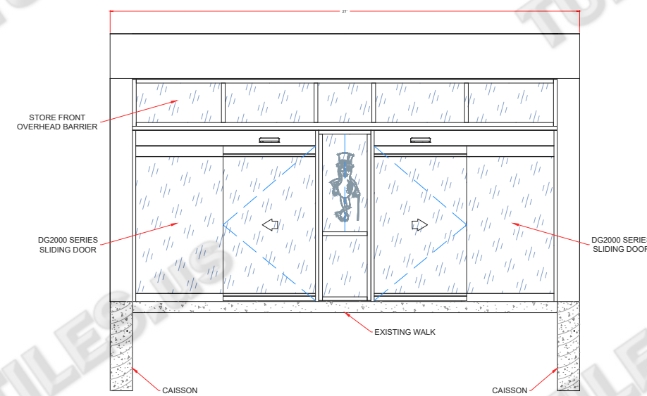
ELEVATION - SLIDING DOORS
