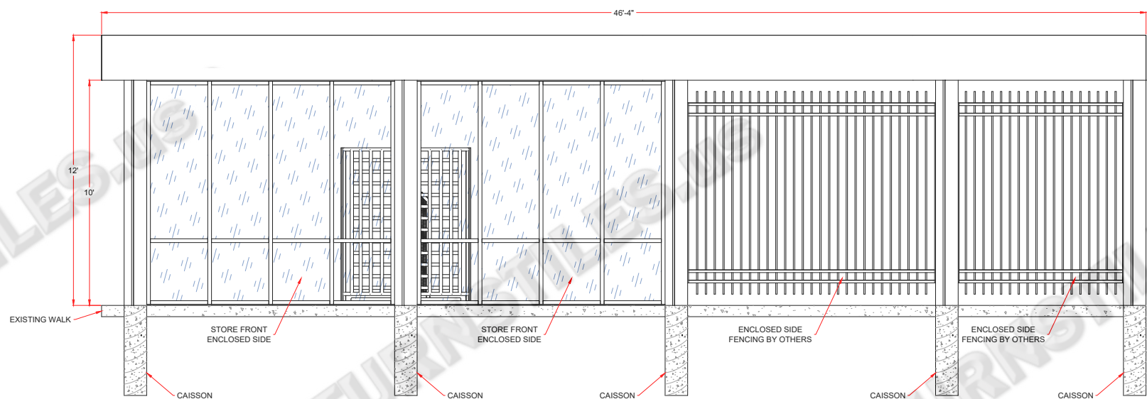
ELEVATION - RIGHT SIDE
