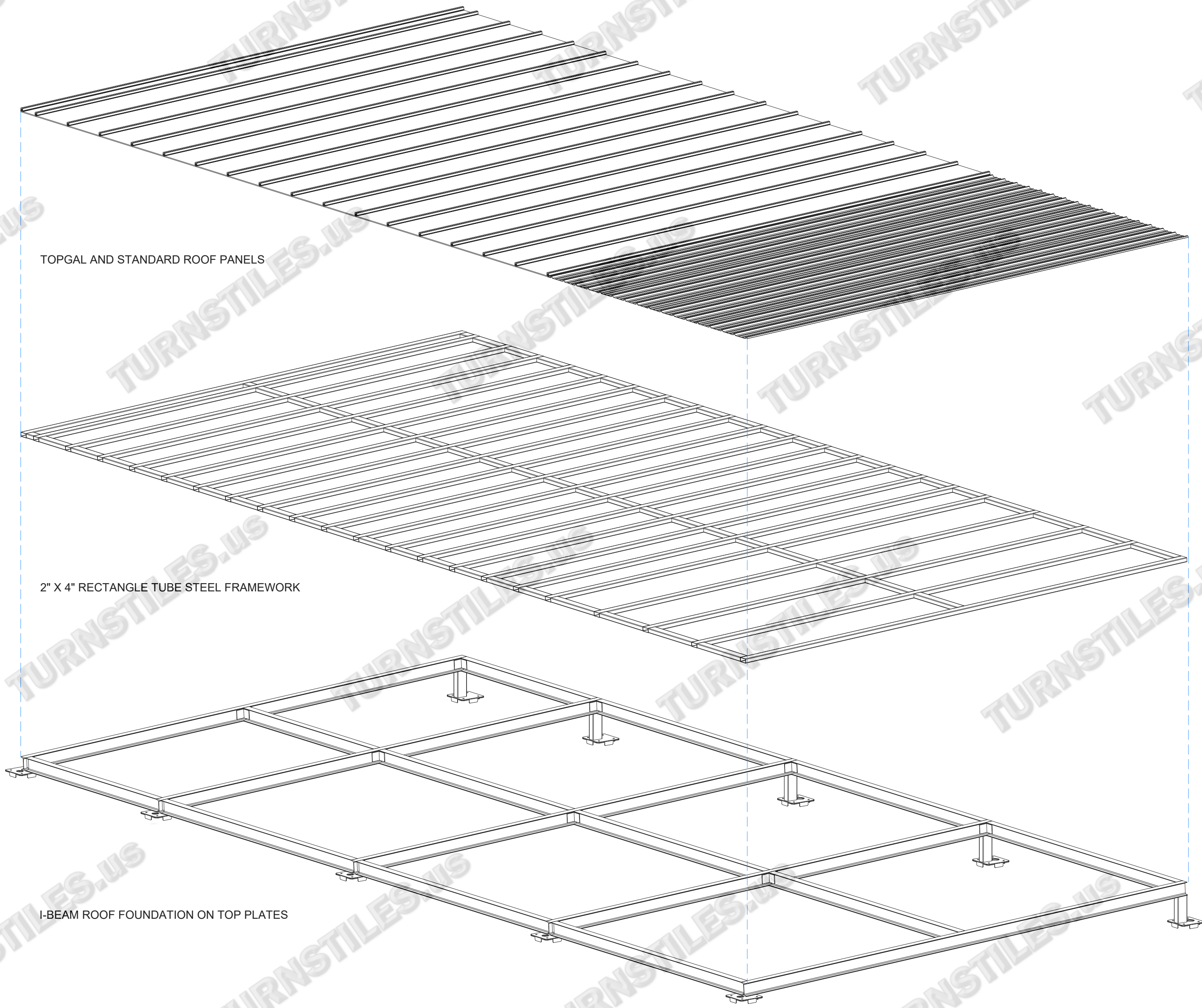
ROOF - OVERHEAD EXPLODED DETAIL
