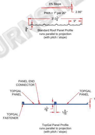
ROOFING TYPE(S) - PROFILES - DETAILS
