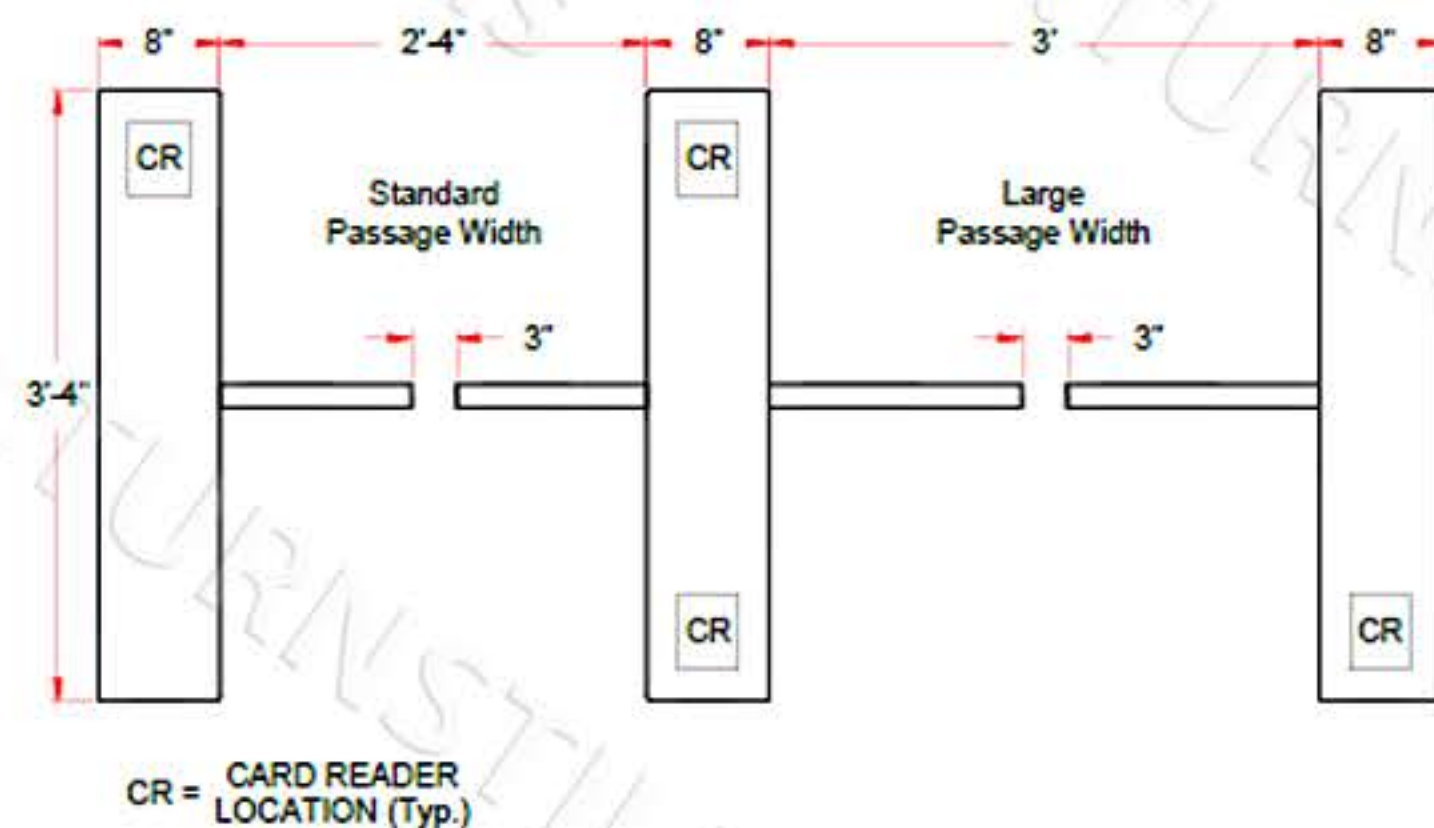
CABINET TOP VIEW
