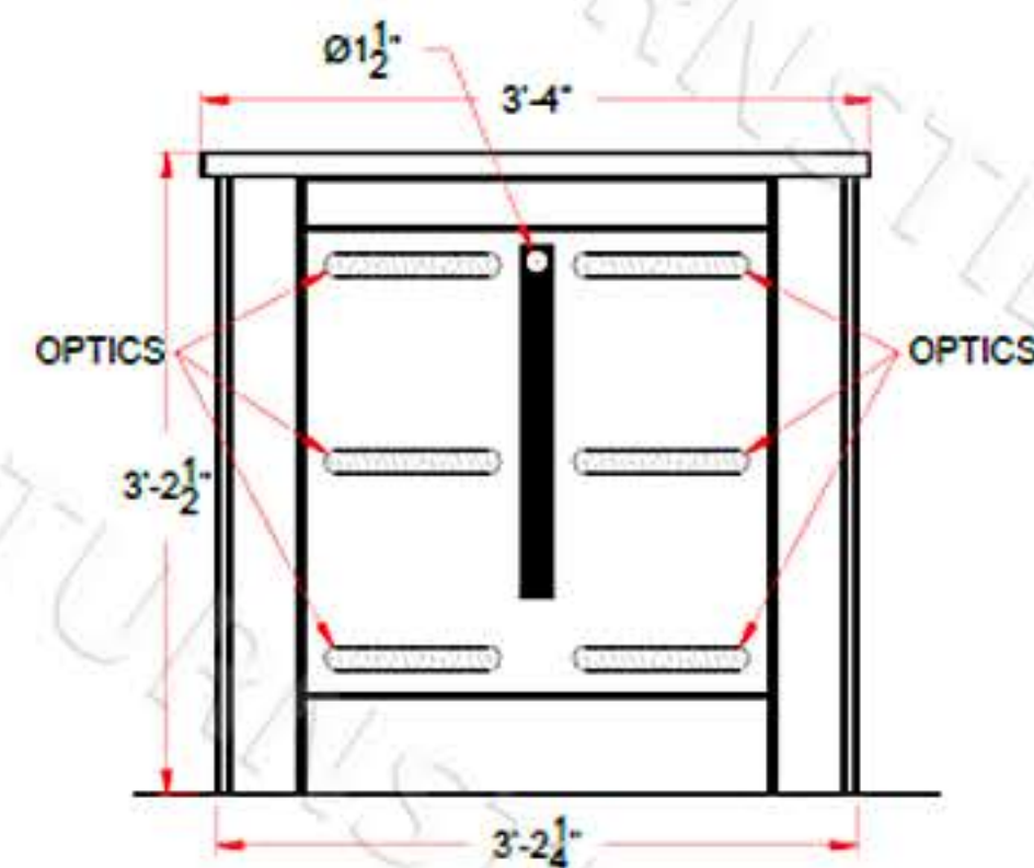
ELEVATION CABINET INNER FACE
