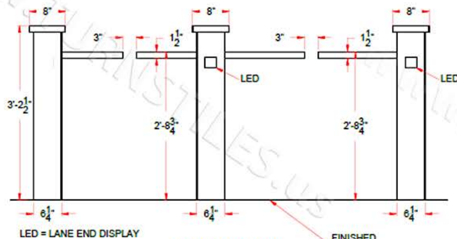
ELEVATION PASSAGE WIDTHS
