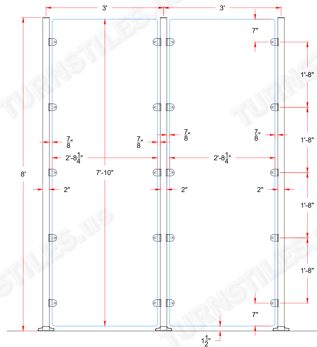
ELEVATION Typical example of two sections, 3' Wide - On Center
