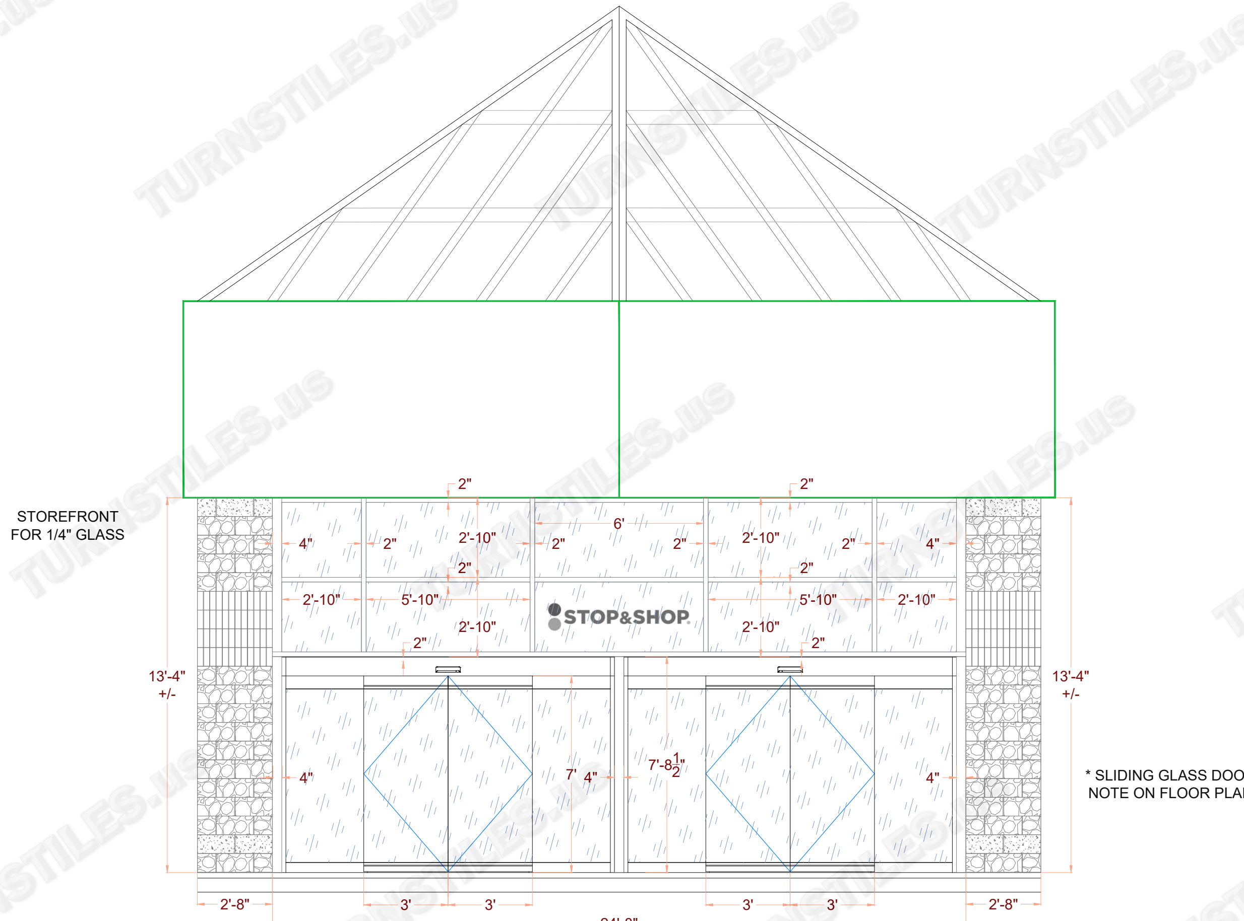
FRONT ELEVATION
