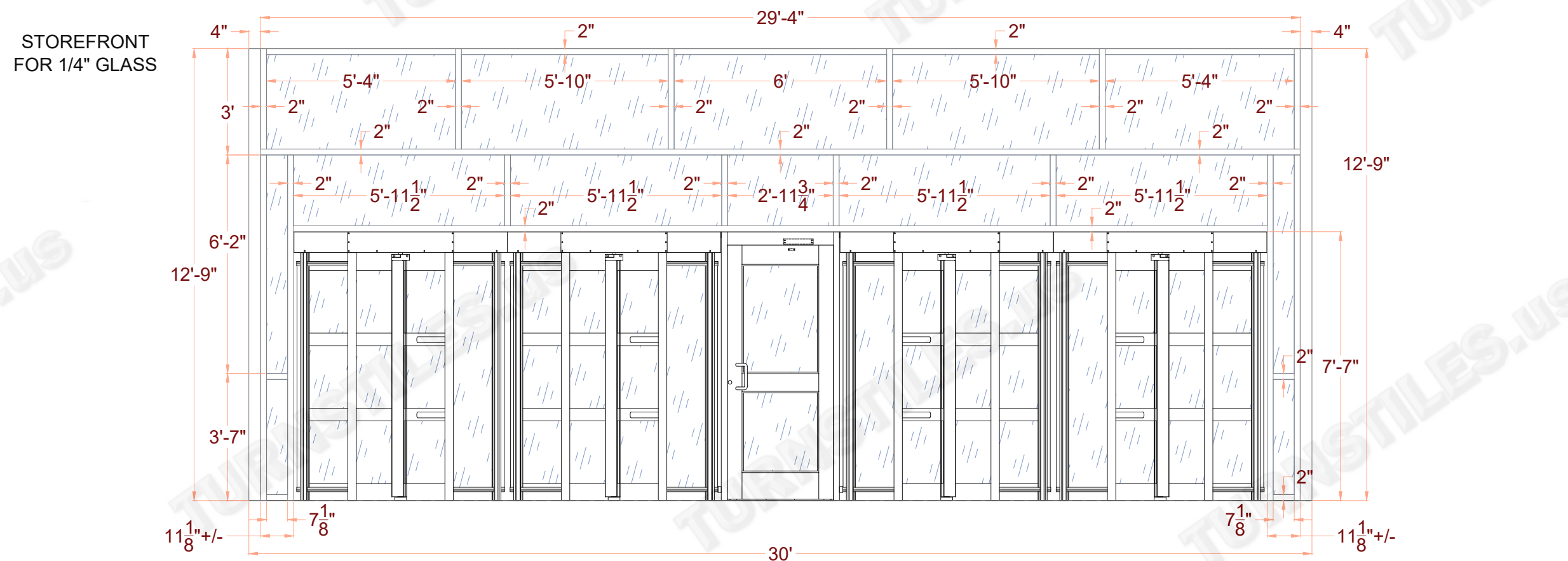
INTERIOR ELEVATION
