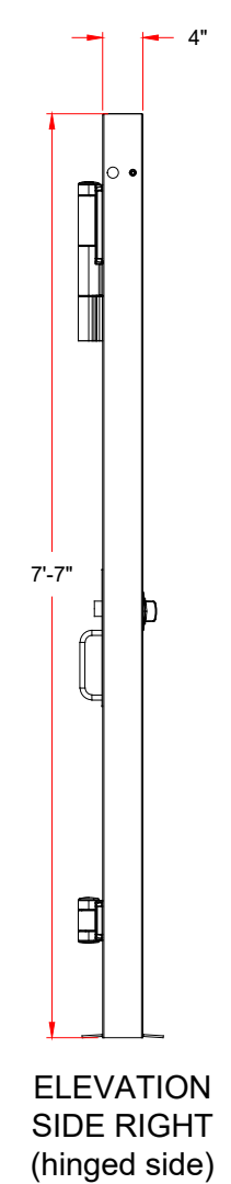
AG36ADA Swing Gate Detail and Dimensions
