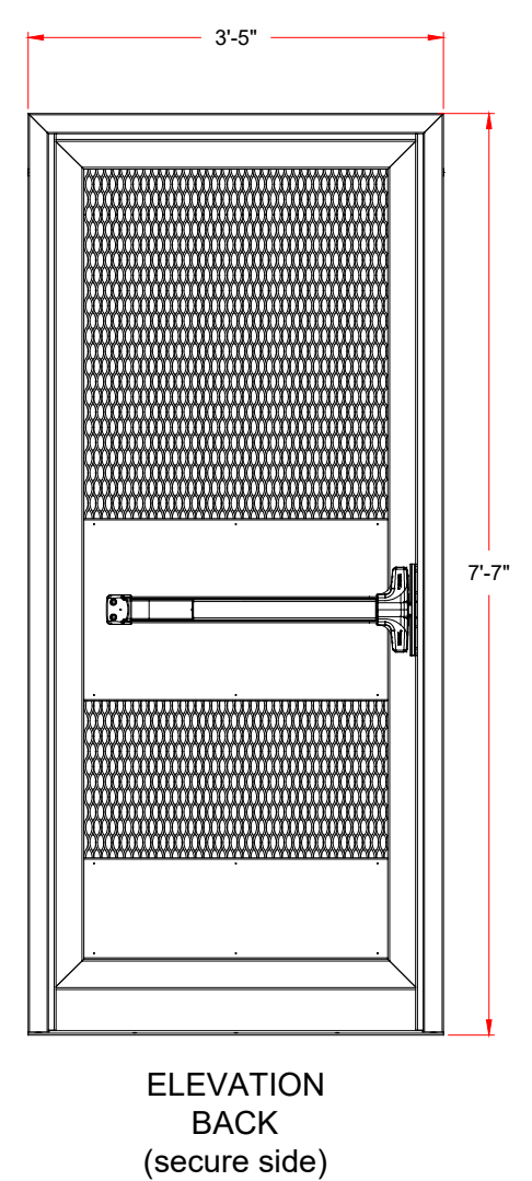
AG36ADA Swing Gate Detail and Dimensions
