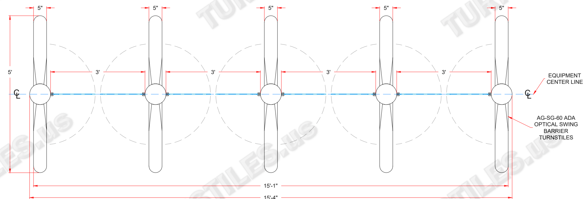
SECURE SIDE SOUTH LOBBY FLOOR PLAN
