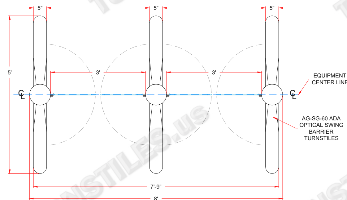
SECURE SIDE NORTH LOBBY FLOOR PLAN
