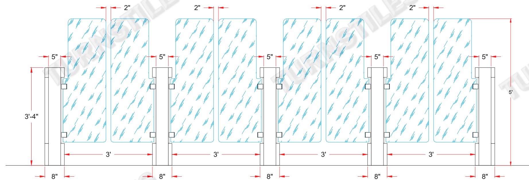
ELEVATION SOUTH LOBBY
