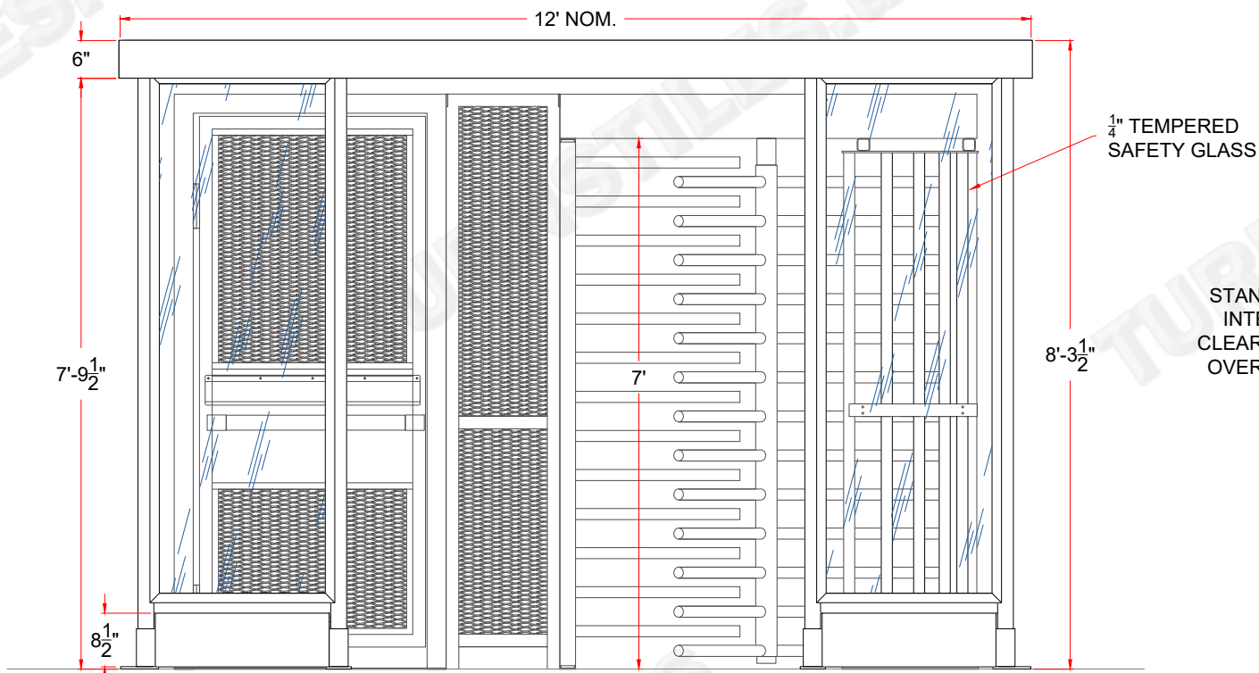
ELEVATION - REAR SECURE SIDE
