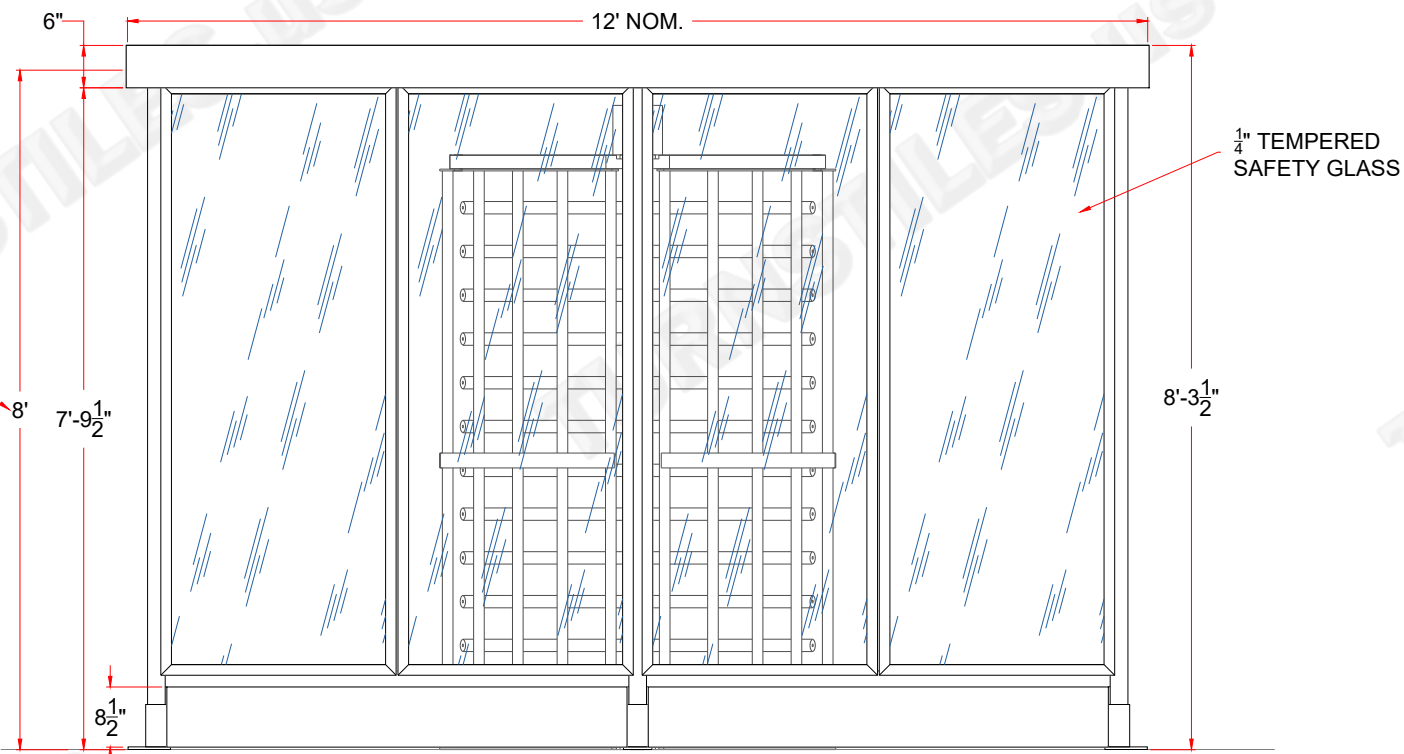
ELEVATION - SIDE
