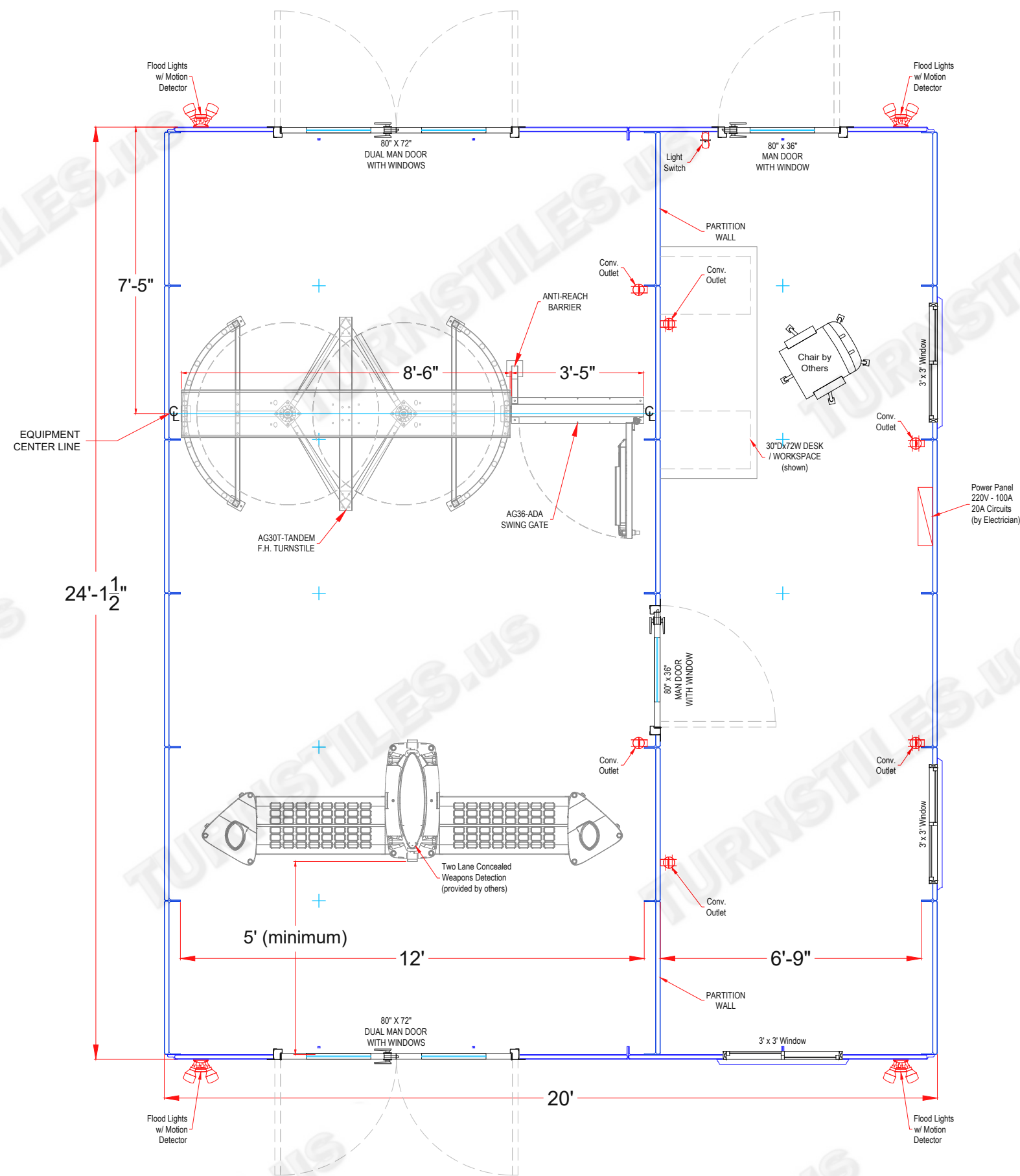
EQUIPMENT FLOOR PLAN
