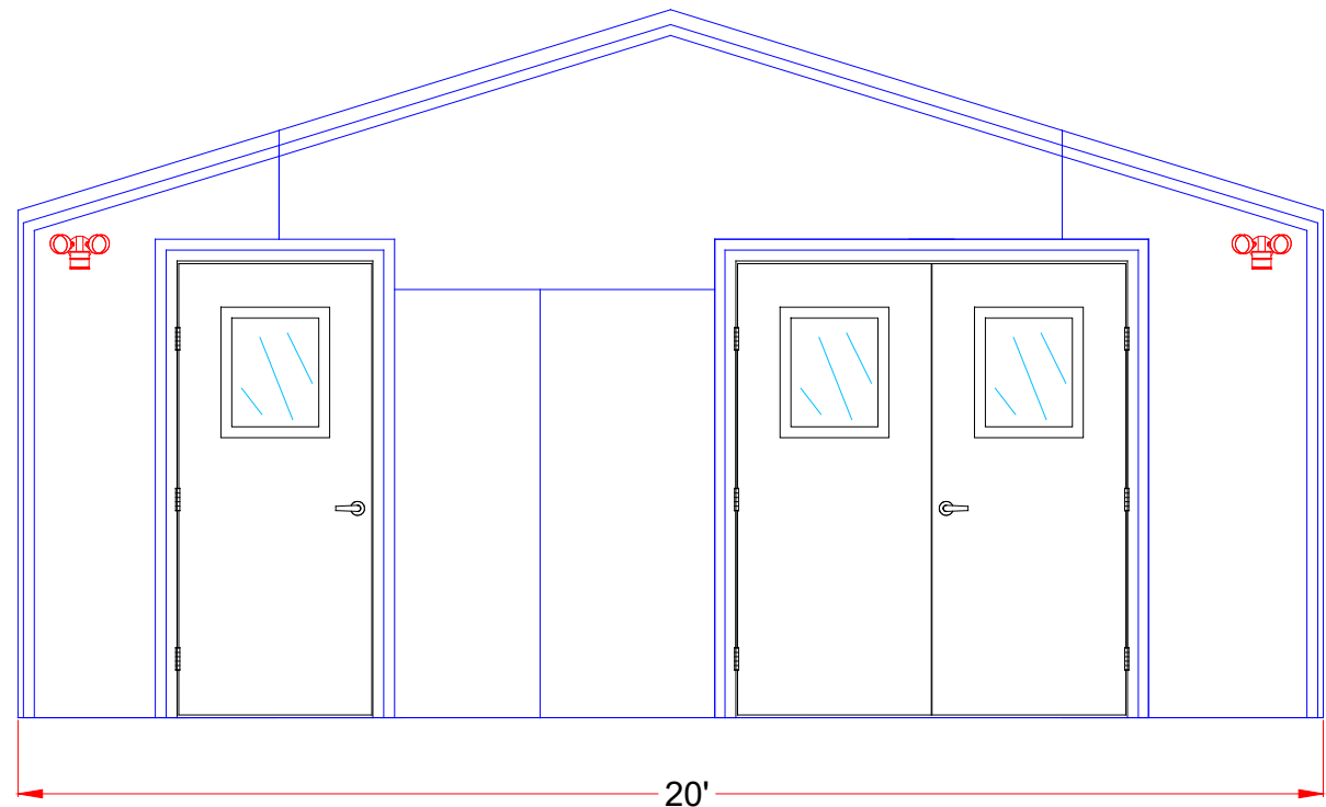
REAR ELEVATION SECURE SIDE
