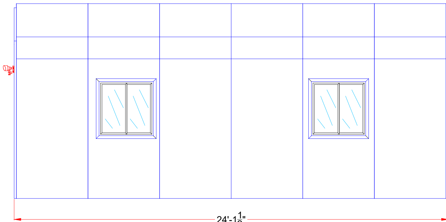
ELEVATION RIGHT SIDE (Electrical connection and HVAC not shown)
