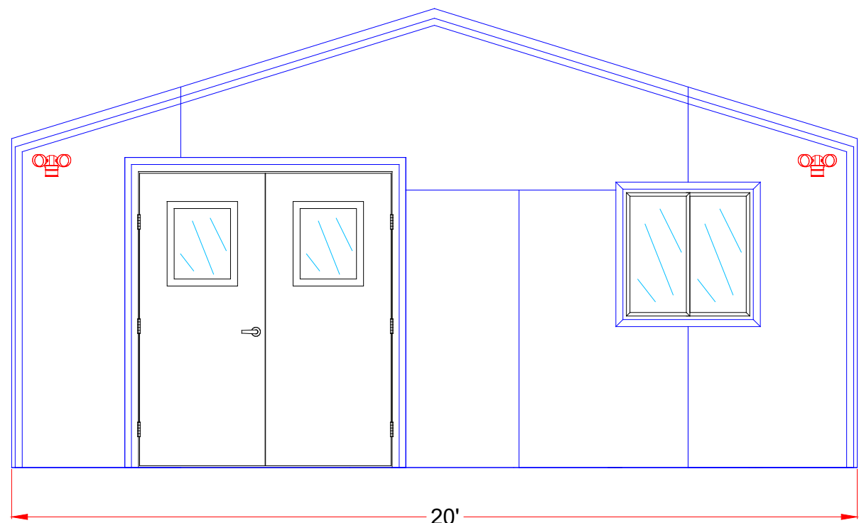
FRONT ELEVATION NON SECURE SIDE
