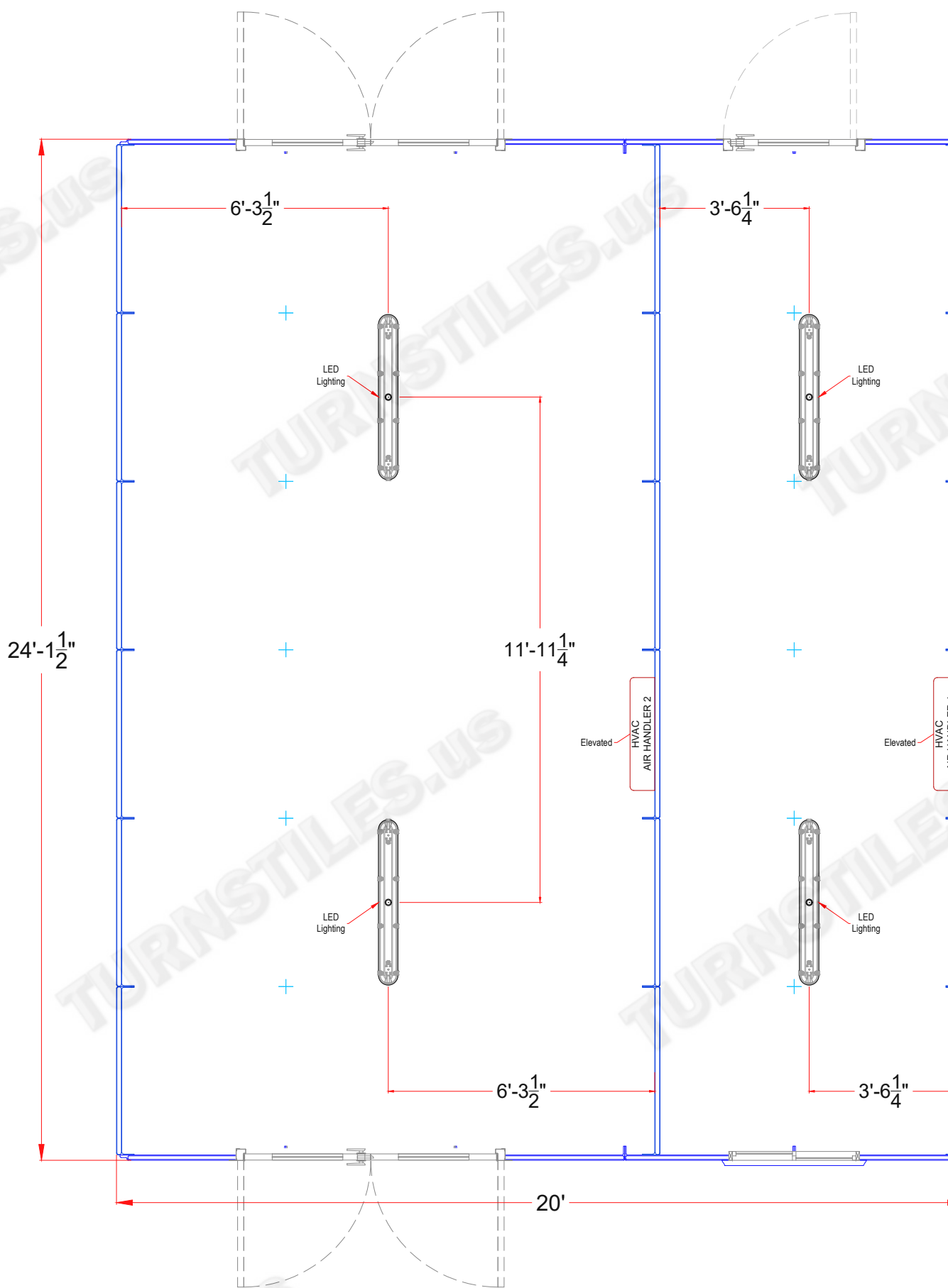
INTERIOR OVERHEAD LIGHTING PLAN AND DUAL SPLIT HVAC SYSTEM
