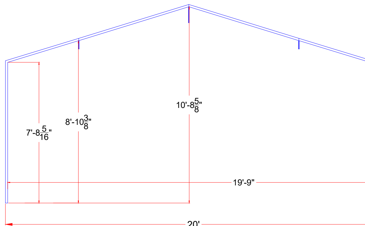
INTERNAL DEPTH DIMENSIONS PAST SIDE PANEL FLANGES
