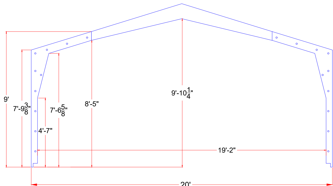
EXTERNAL HEIGHTS AND PANEL FLANGE DIMENSIONS
