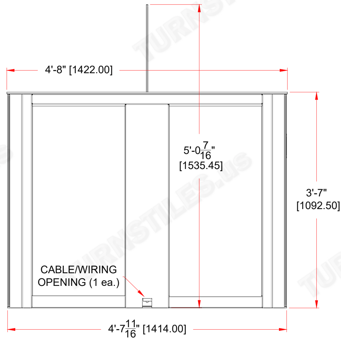
SIDE VIEW
