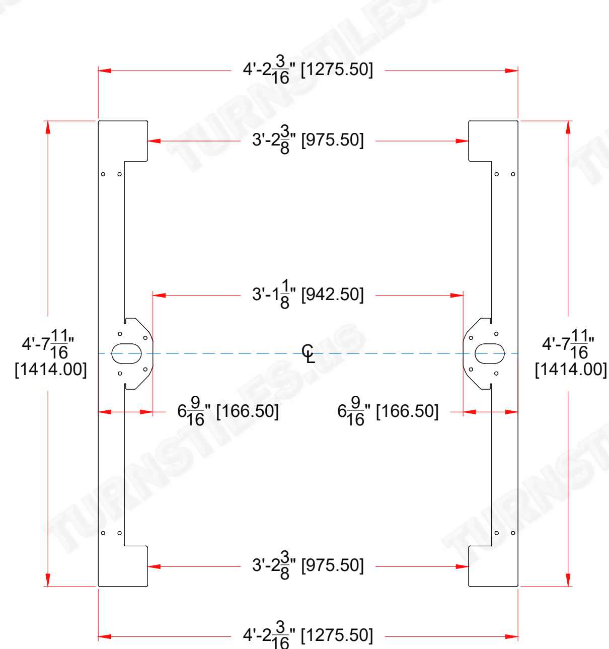
ANCHOR DETAIL Template Layout Dimensions
