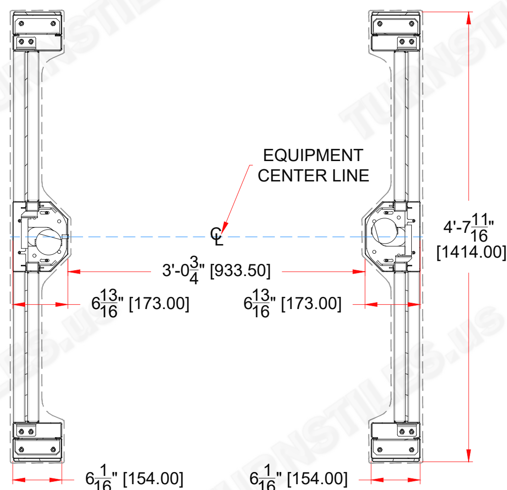
SECTION External Dimensions
