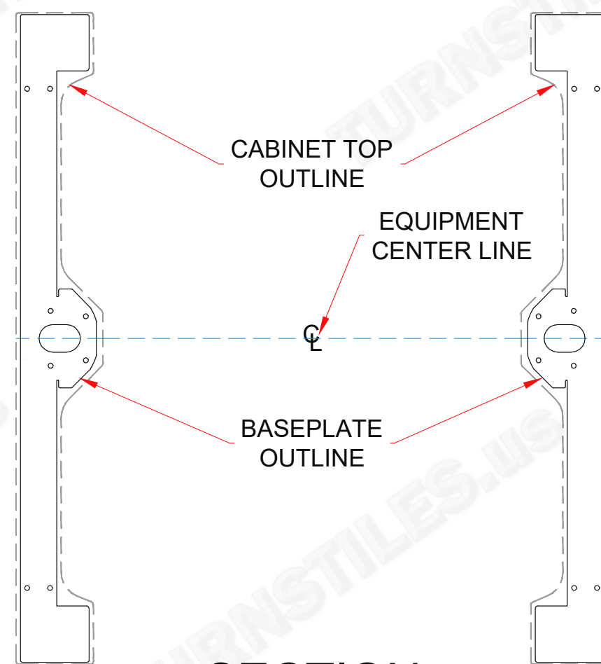
SECTION TOPS/BASES
