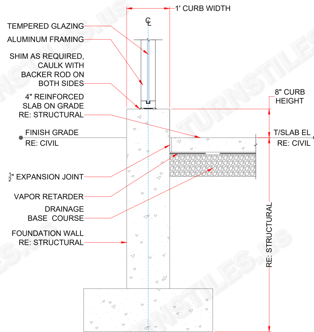
FOUNDATION DETAIL PER USAGE FROM PROVIDED PLANS
