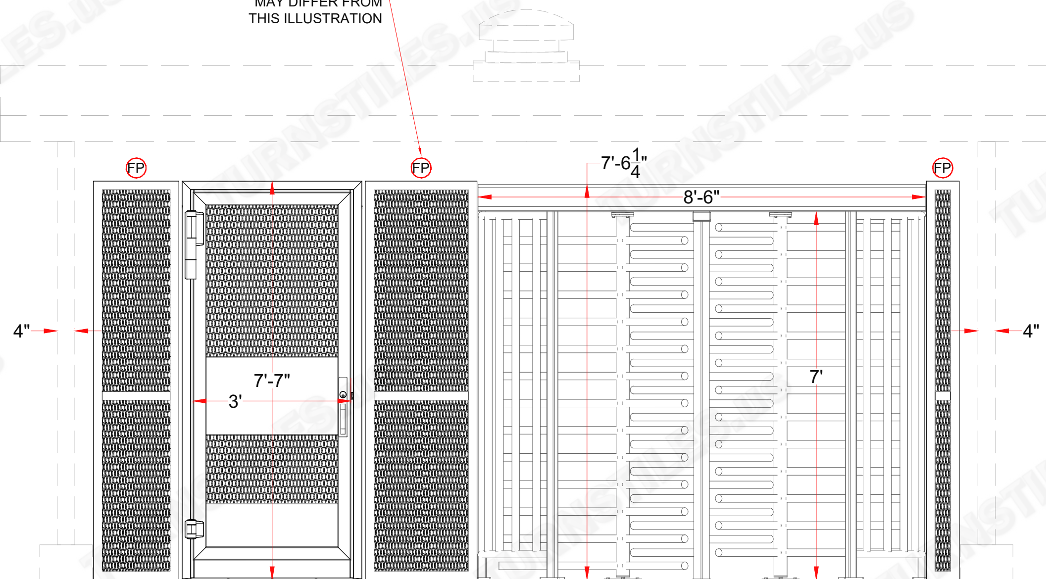
STOREFRONT ENCLOSED CANOPY SECTION - EQUIPMENT AND FILLER PANELS
