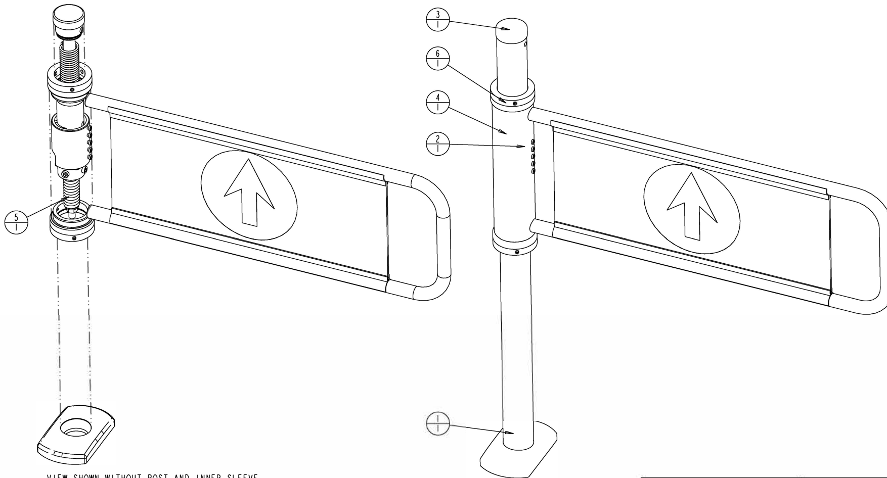
VIEW SHOWN WITHOUT POST AND INNER SLEEVE
