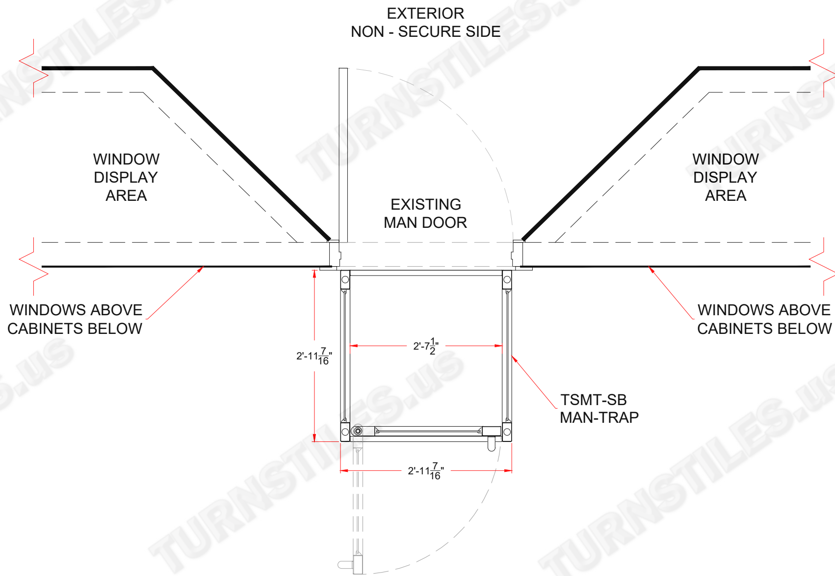
FLOOR PLAN FOOT PRINT - SECURE SIDE
