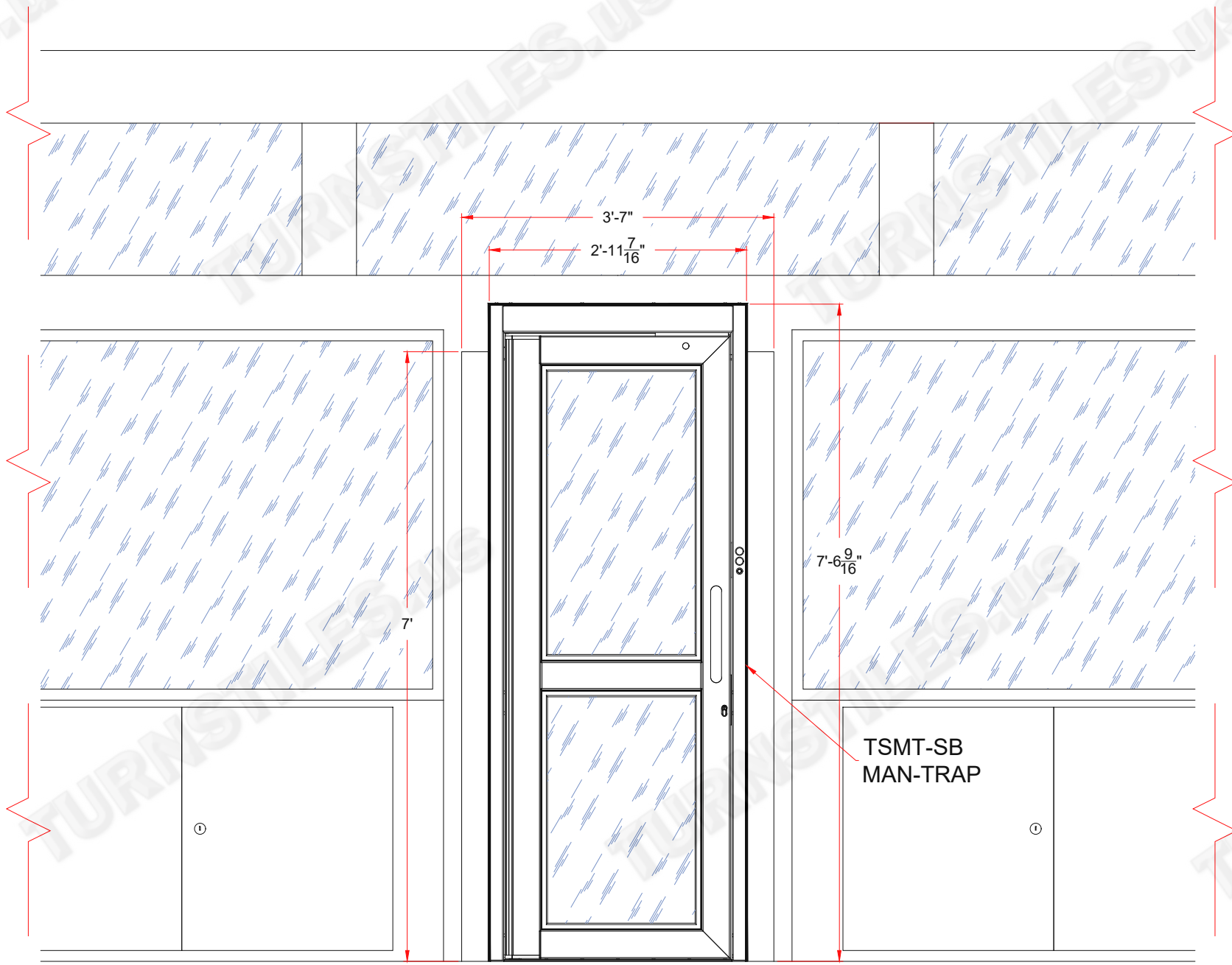
EXIT VIEW ELEVATION INTERIOR - SECURE SIDE
