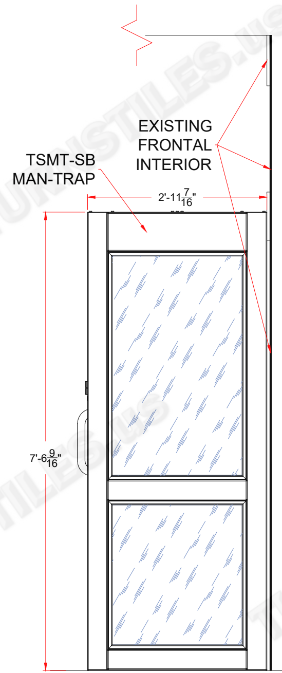
LEFT SIDE VIEW ELEVATION - INTERIOR
