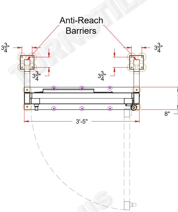
FOOT PRINT
