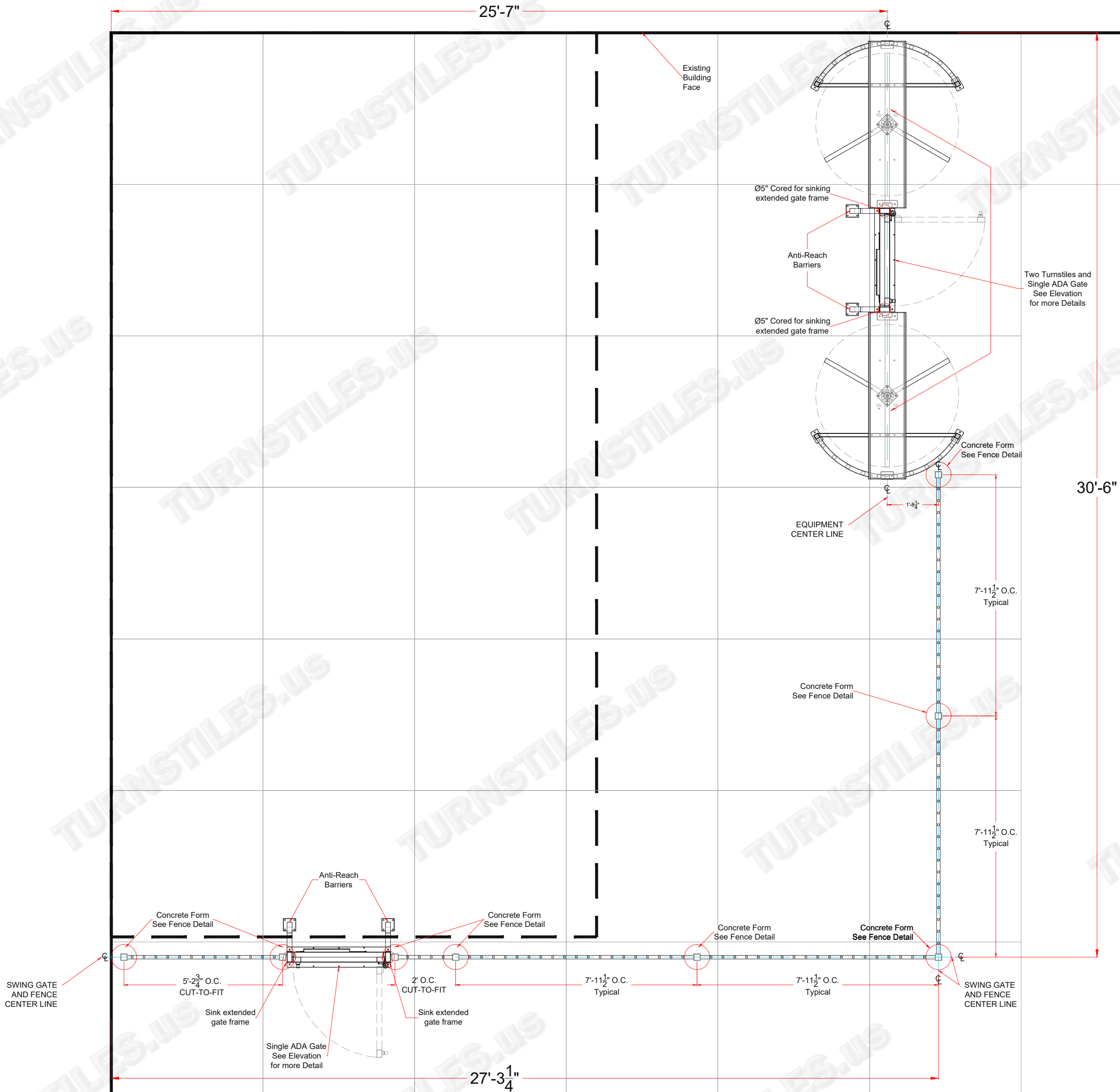
PLAN
