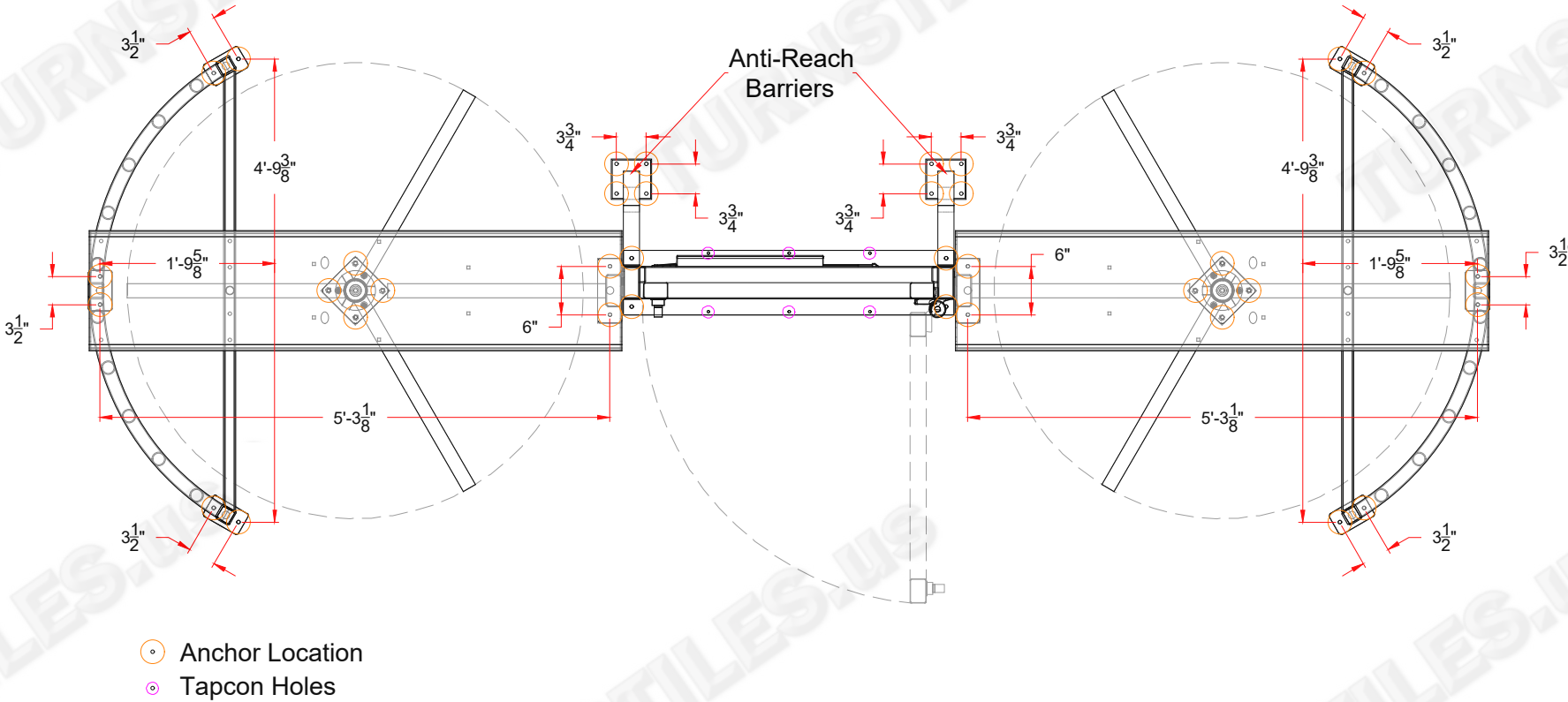
FOOT PRINT
