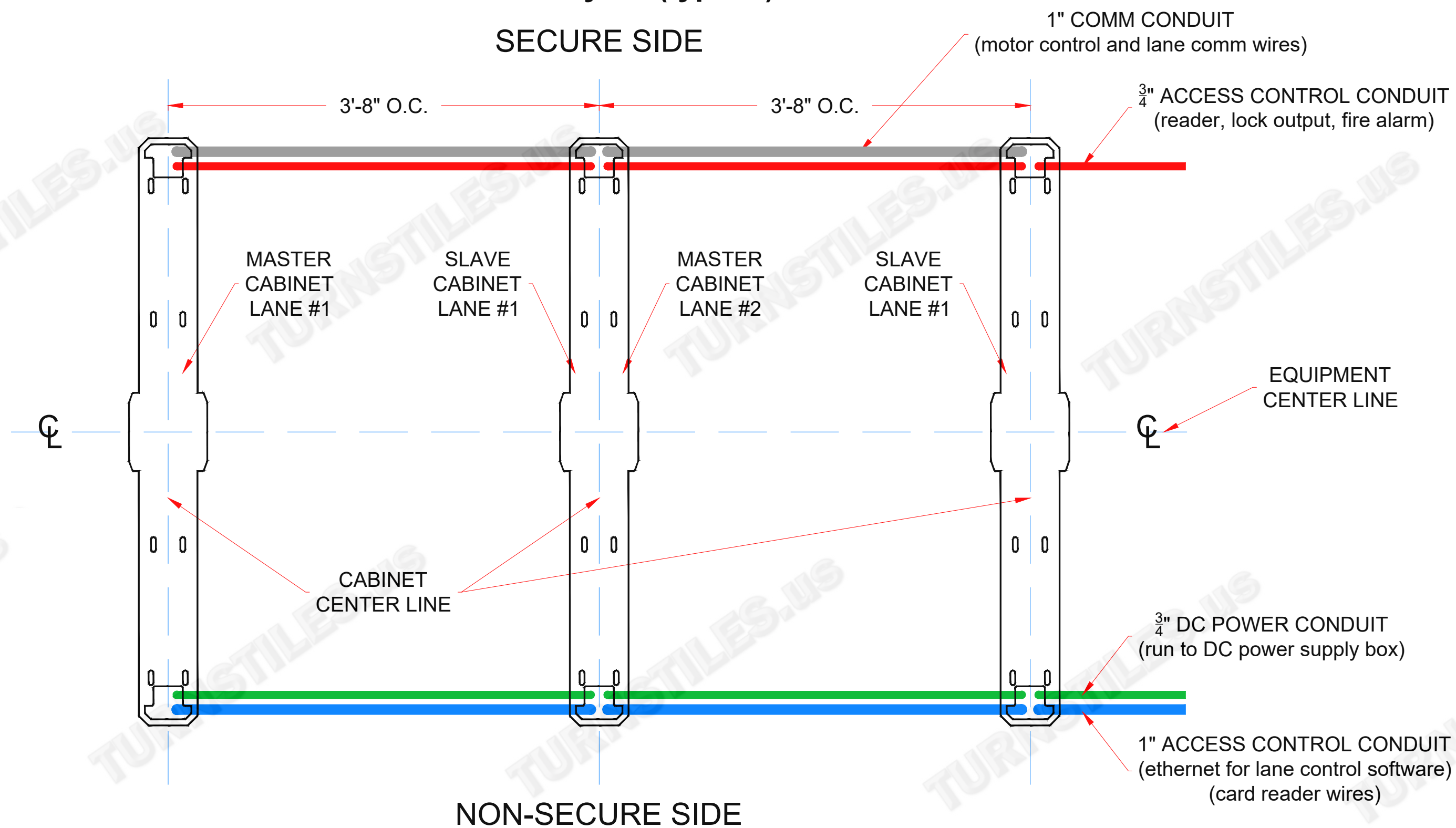
Conduit Layout (typical)
