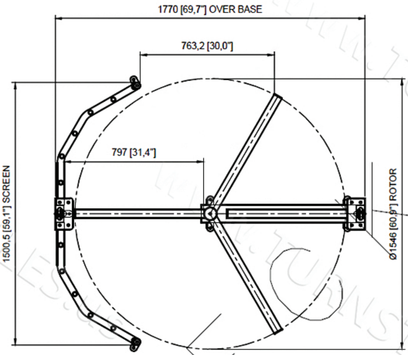
PLAN VIEW (SECTIONED)
