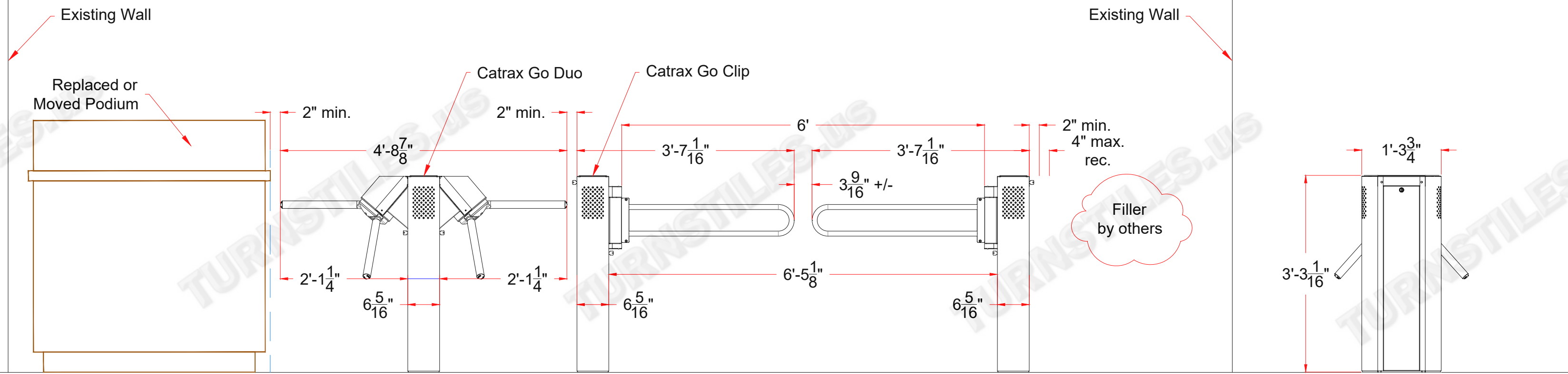
ELEVATION Non-secure Side
