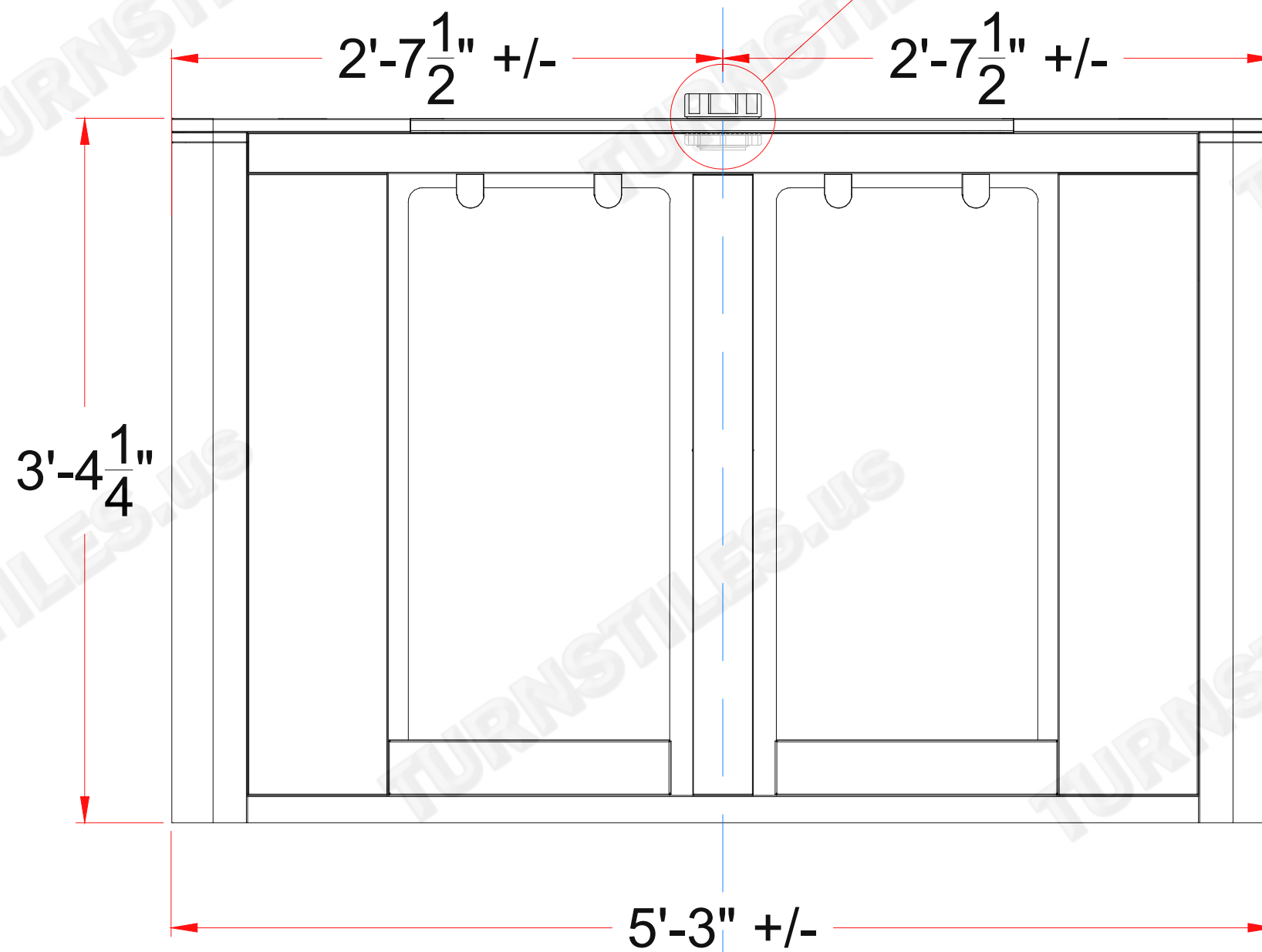
SIDE ELEVATION
