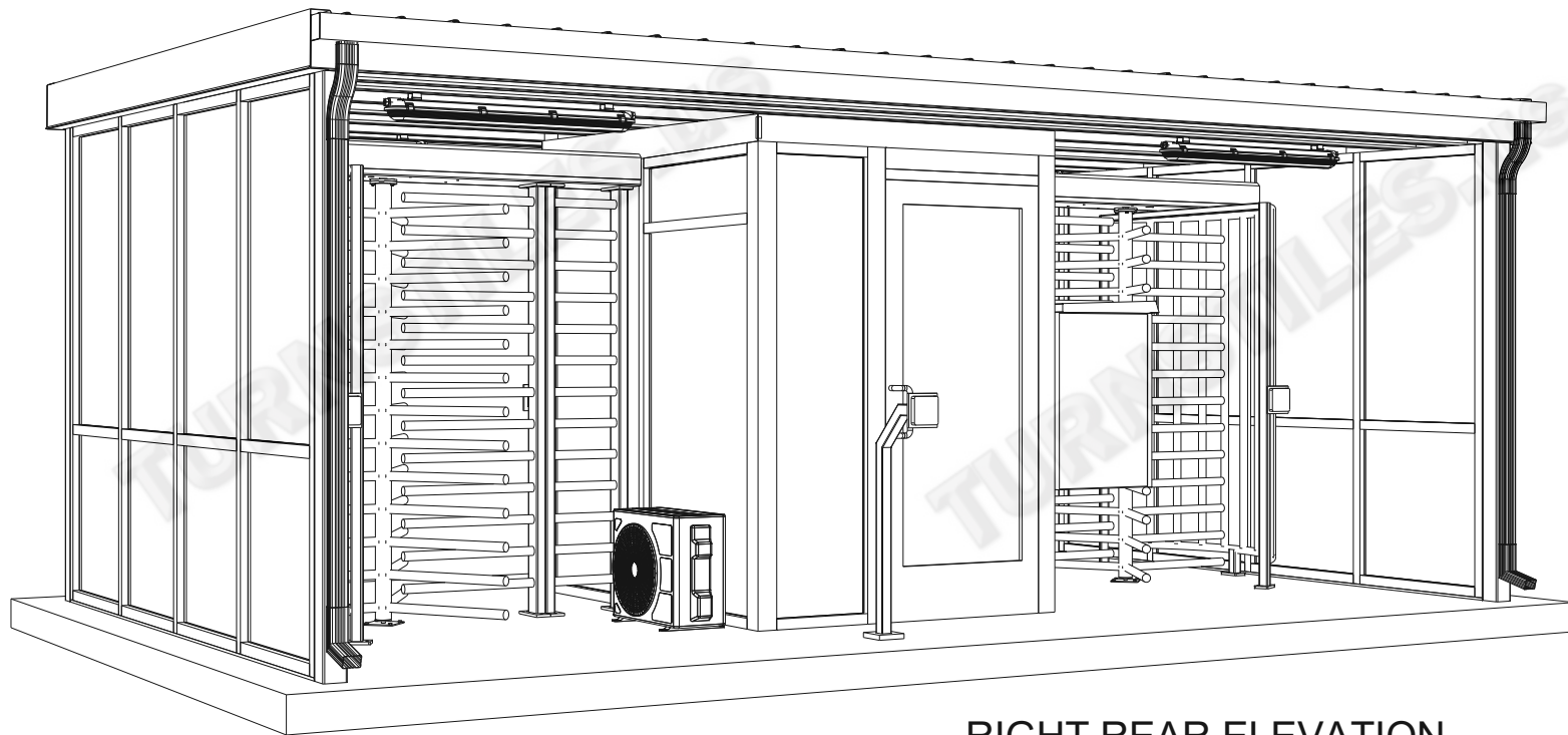
RIGHT REAR ELEVATION NON SECURE SIDE
