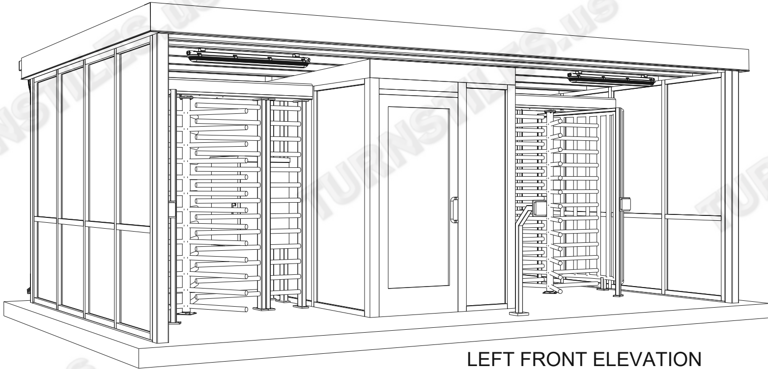
LEFT FRONT ELEVATION SECURE SIDE
