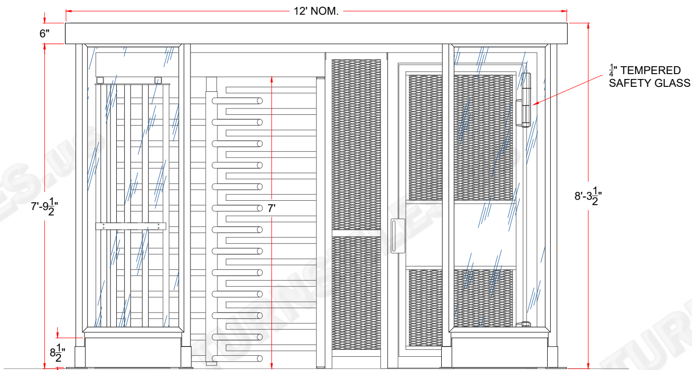
ELEVATION - FRONT NON-SECURE SIDE
