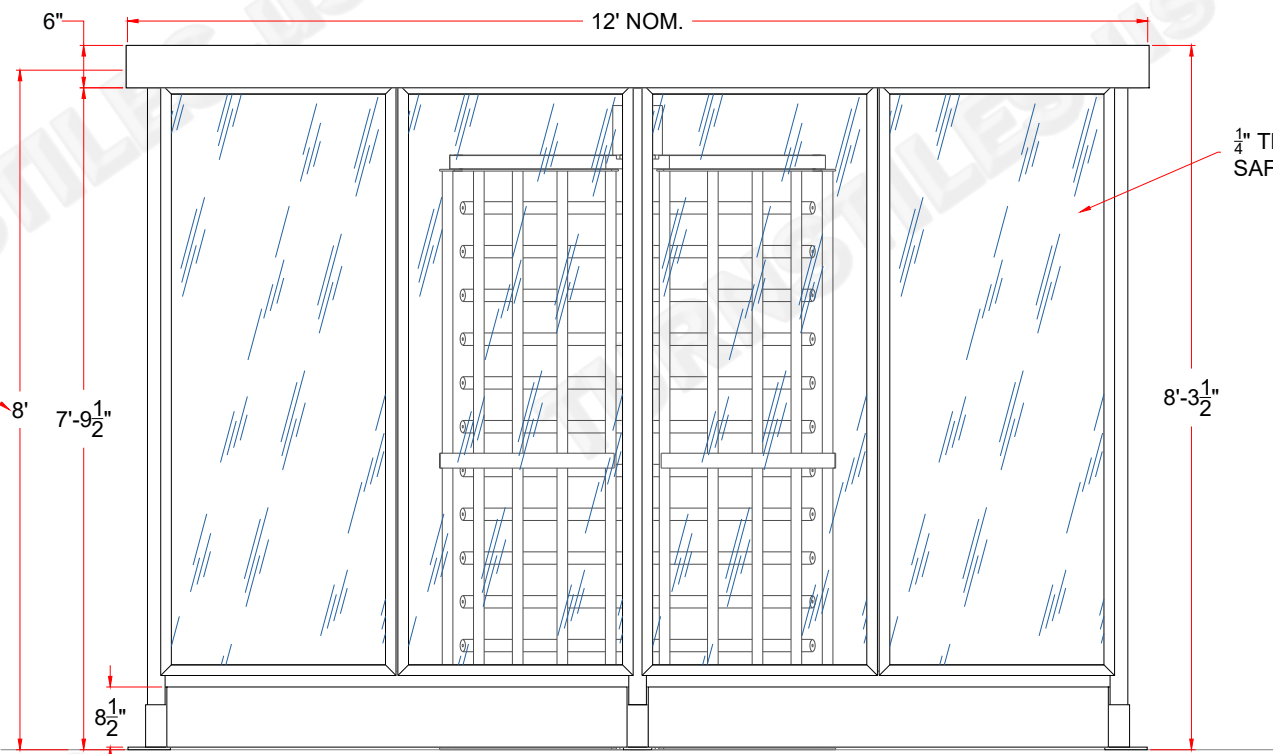
ELEVATION - SIDE
