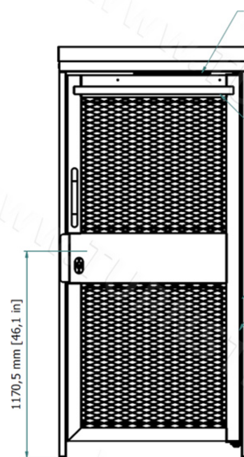
BACK
