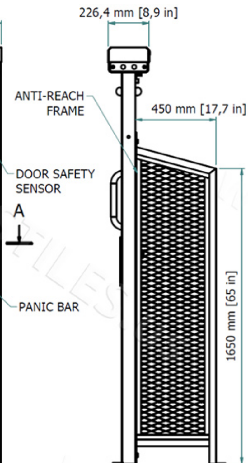
SIDE (L)
