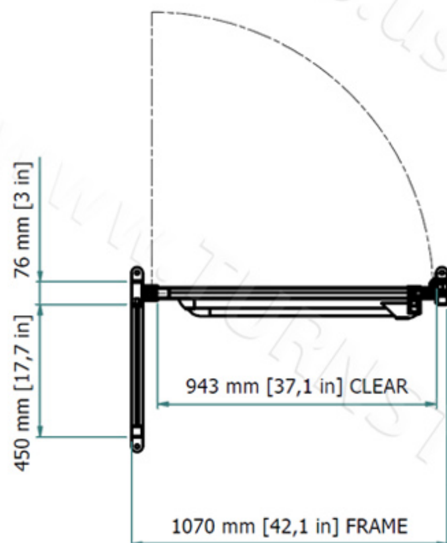
SECTION: A-A
