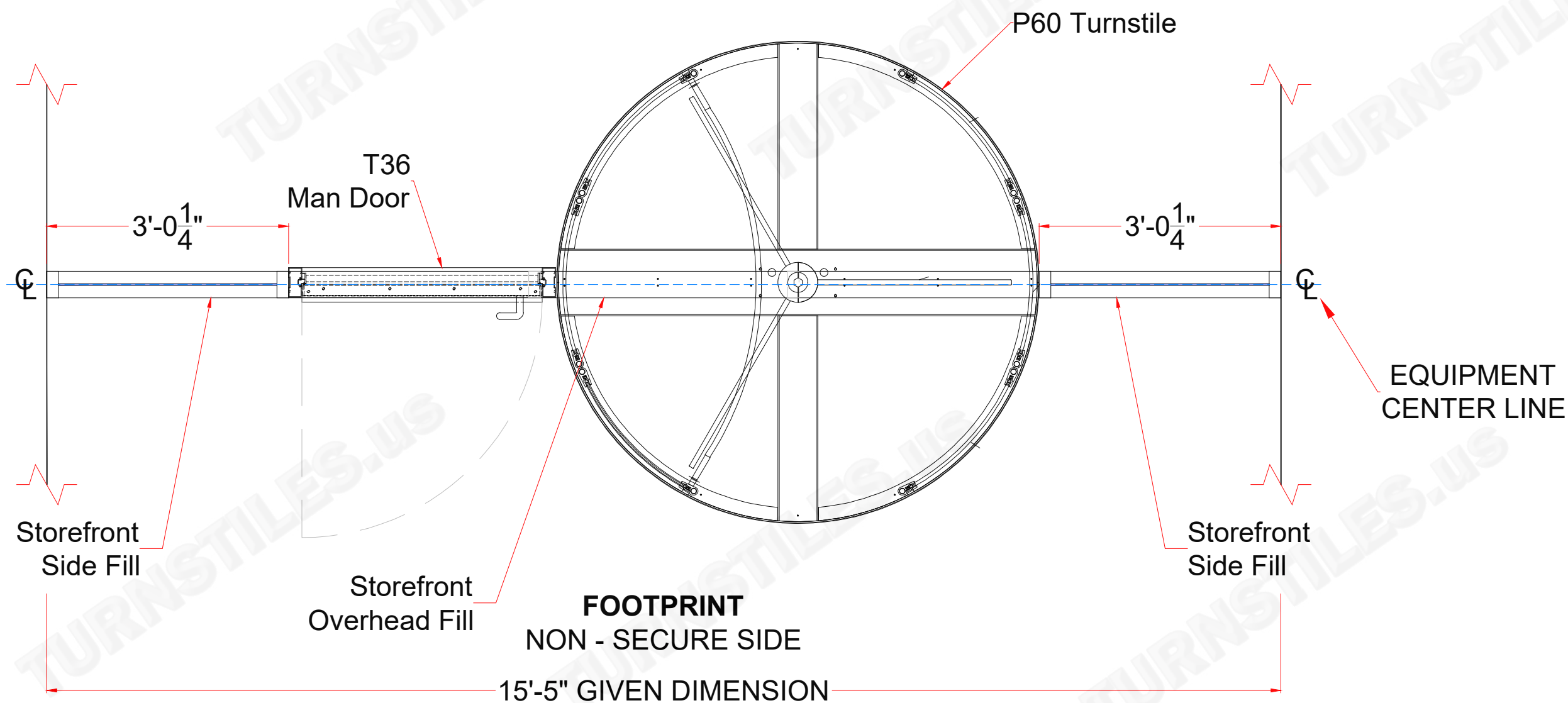
FOOTPRINT NON - SECURE SIDE
