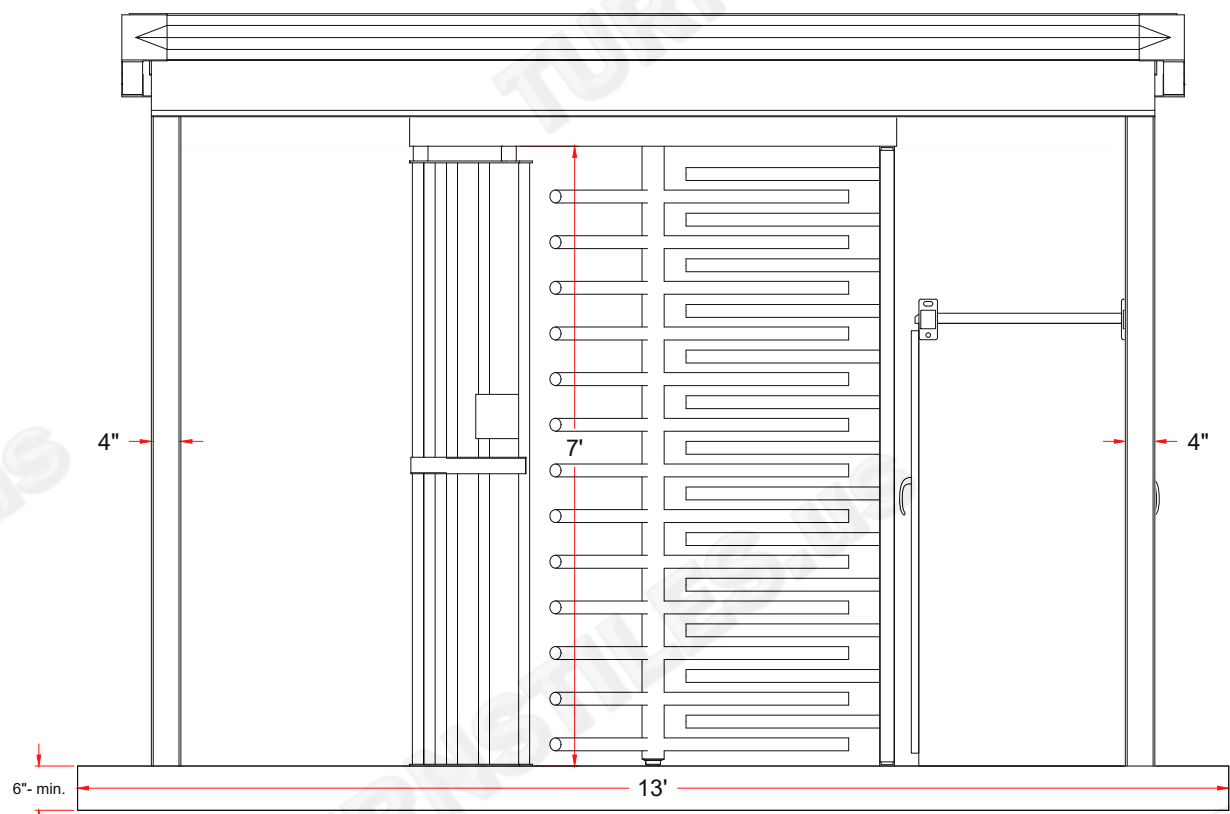
ELEVATION - SECURE SIDE (panels not shown)
