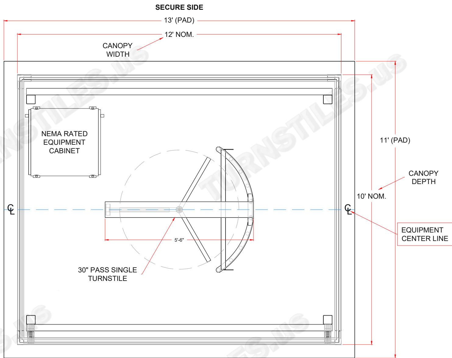
FOOT PRINT NON SECURE SIDE (flat pan not shown)
