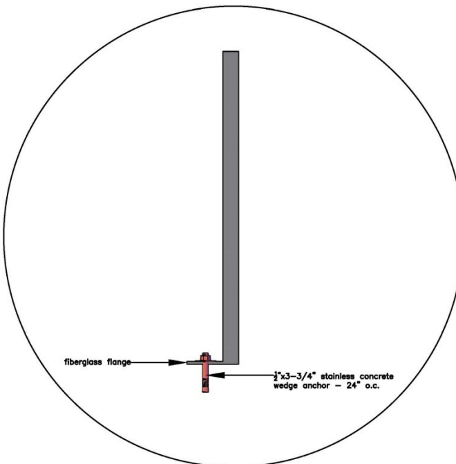
Fiberglass flange
