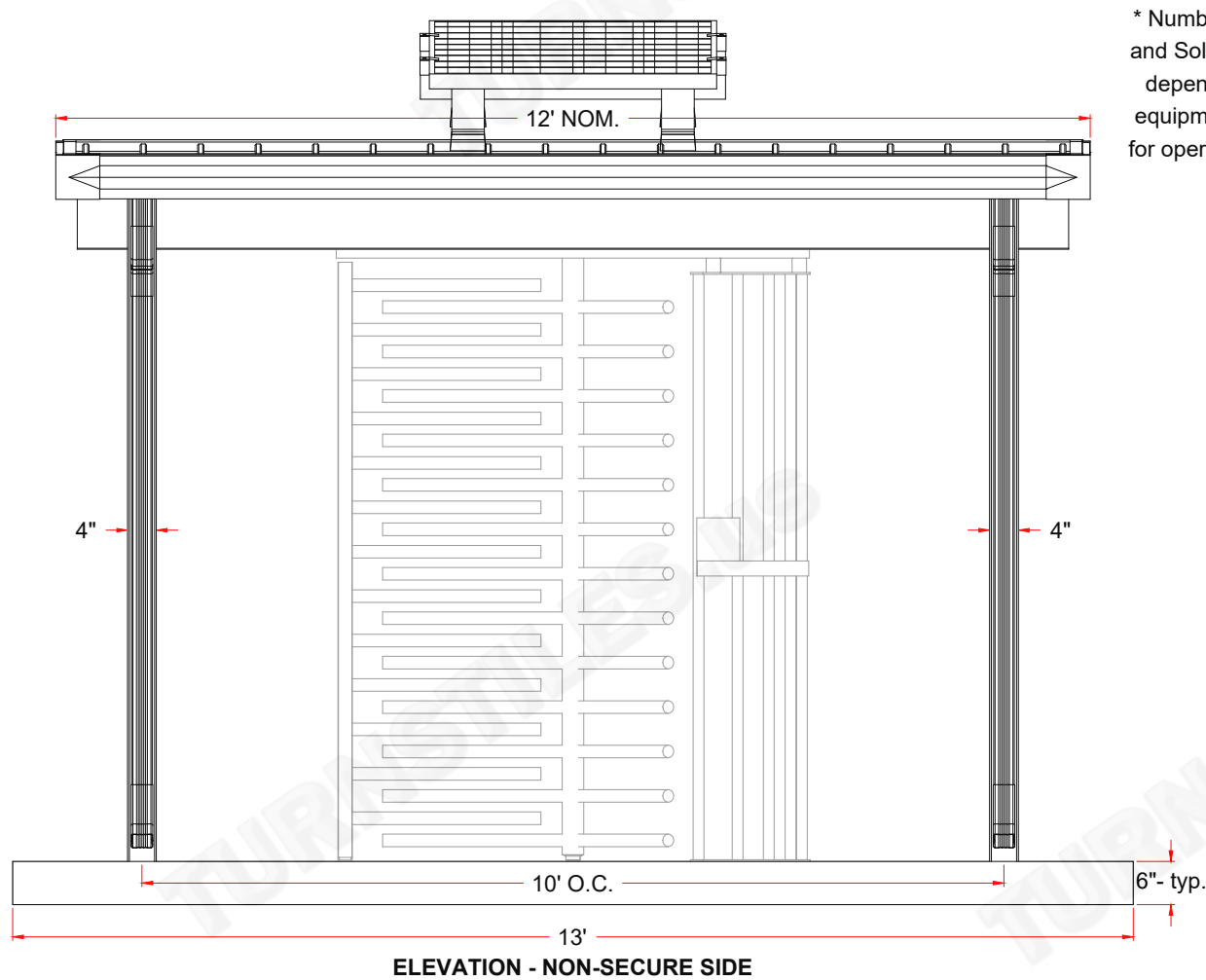
ELEVATION - NON-SECURE SIDE
