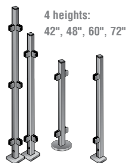
Receiver Post
