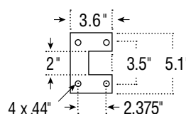
Cut Flange
