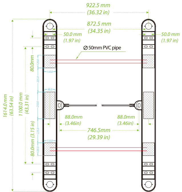
Bottom View
