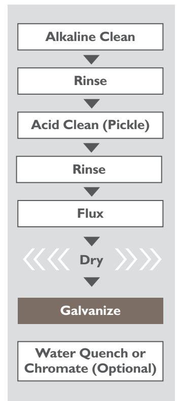
Figure 4: Dry galvanizing process
