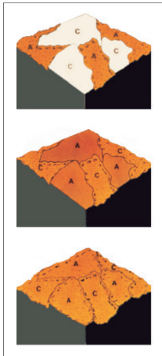
Figure 3: Changes in anodic and cathodic areas
